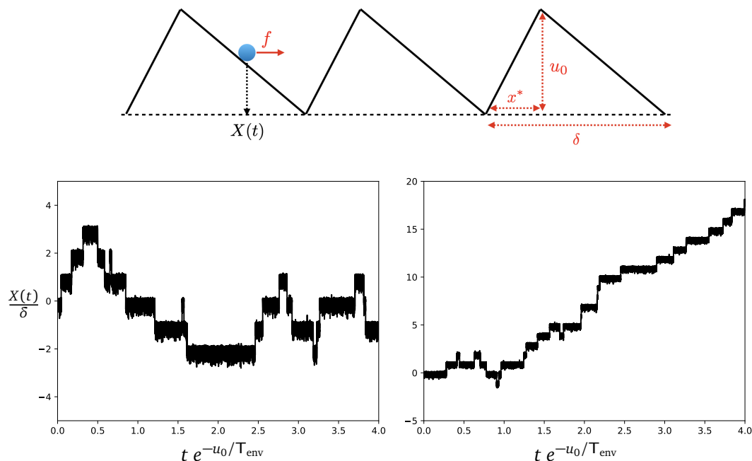
Figure 1: Nonequilibrium version of Kramer's model exhibiting an increased reaction rate due to nonequilibrium driving. Trajectories shown are for a reaction coordinate X that solves the Langevin equation \partial_t X(t) = (f - \partial_x u(X(t)))/\gamma + \sqrt{2T_{\text{env}}/\gamma} \xi(t) , where \xi(t) = dW(t)/dt is a delta-correlated white Gaussian noise term, and where u(x) is a triangular potential with period \delta , i.e. u(x) = u(\pm\delta) , u(x) = u_0 x/x^* if x \in [0, x^*] , and u(x) = u_0(\delta - x)/(\delta - x^*) if x \in [x^*, \delta] . Left: equilibrium trajectory with f = 0 . Right: nonequilibrium trajectory with f \delta/T_{\text{env}} = 1 . The remaining parameters are set to \delta = 5 , \gamma = 1 , x^* = 1 , u_0 = 10 , and T_{\text{env}} = 1 .
