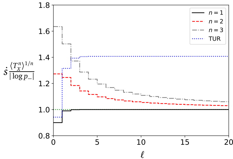
Figure 5: Comparing the tightness of the first-passage time bounds Eq. (3) with the thermodynamic uncertainty relation Eq. (59). The ratio \dot{s} \langle T_X^n \rangle^{1/n} / |\log p_-| for n = 1, 2, 3 and the thermodynamic uncertainty (TUR) ratio \dot{s}(\langle T_X^2 \rangle - \langle T_X \rangle^2) / (2\langle T_X \rangle) are plotted as a function of \ell = \ell_- = \ell_+ for a biased random walk process X described by Eq. (73) with k_+ = 1 and b = 0.1 . Note that the inequalities Eq. (3) are tight for \ell \rightarrow \infty , while the uncertainty relation Eq. (59) is loose.
