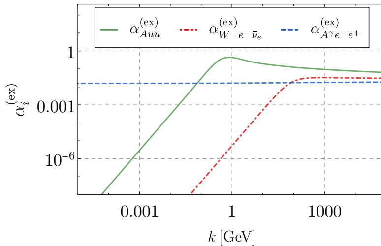
Figure 13: The exchange couplings of the quark-gluon coupling \alpha_{Au\bar{u}}^{(ex)} (green, solid), the electron- W^\pm coupling \alpha_{W^\pm e^-\bar{\nu}_e}^{(ex)} (red, dash-dotted), and the photon-electron coupling \alpha_{A\gamma e^-e^+}^{(ex)} (blue, dashed) as defined in (C.21) and (C.31). The decrease of the strong and weak coupling towards small momenta is triggered by the QCD mass gap and the mass of the W boson, respectively. The electromagnetic coupling does not decrease in the IR due to the absence of a photon mass.
