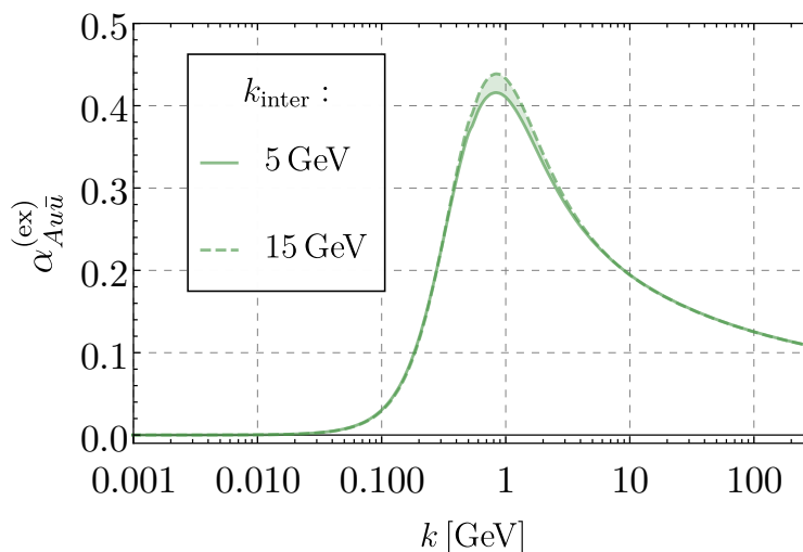
Figure 12: The quark-gluon exchange coupling \alpha_{Au\bar{u}}^{(ex)} defined in (C.21) as a function of k for interface scales k_{inter} = 5, 15 GeV. The chosen k_{inter} does not affect severely the IR dynamics.
