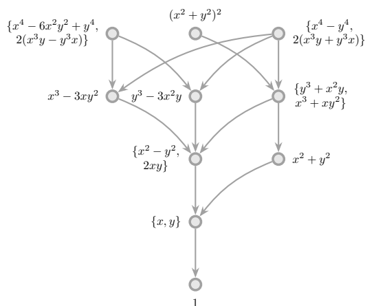
Figure 4: Mixing of irreps of the point group D_6 by translation symmetry for the triangular lattice. Every arrow means that some (infinitesimal) translation acting on the polynomial(s) of higher degree generates the polynomial(s) of lower degree. As for the square lattice, all multipole groups that contain a polynomial of degree n \geq 2 must also include both components of dipole, and charge. The representations of the polynomials under the point group are given in Table 2.
