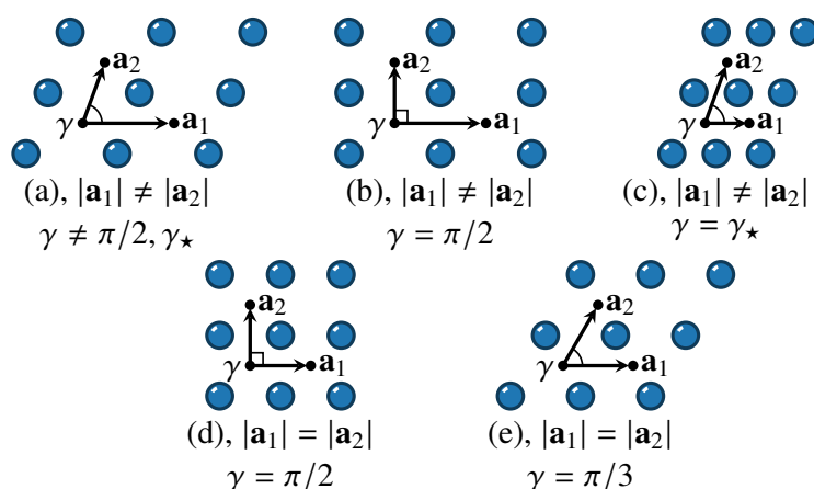
Figure 1: Illustration of the five Bravais lattices in two spatial dimensions. The lattice translation vectors \mathbf{a}_1 and \mathbf{a}_2 are denoted by black arrows, which make an angle \gamma with one another. (a) Monoclinic, with point group C_2 , (b), (c) orthorhombic, with point group D_2 [in (c), 2|\mathbf{a}_2| \cos \gamma_* = |\mathbf{a}_1| ; alternatively, there exists rectangular unit cell that is not primitive], (d) square, with point group D_4 , and (e) triangular ( \gamma = \pi/3 ), with point group D_6 .
