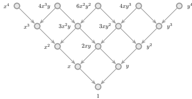
Figure 2: Mixing of monomials under lattice translations for the monoclinic and orthorhombic Bravais lattice types. Every arrow means that some (infinitesimal) translation acting on the monomial of higher degree generates the monomial(s) of lower degree. That is, if a particular monomial is included in the multipole group, compatibility with space group operations requires the multipole group to contain all lower-order monomials that can be reached by following an arrow from the original monomial. Linear combinations of degenerate irreps must be dealt with separately, as described in the main text.
