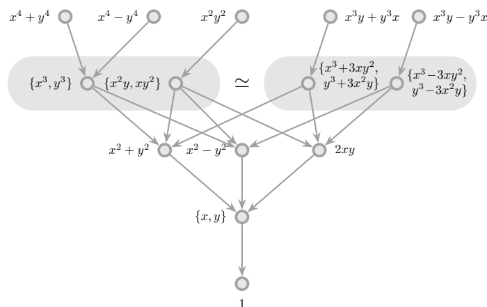
Figure 3: Mixing of irreps of the point group D_4 by translation symmetry for the square lattice. Every arrow means that some (infinitesimal) translation acting on the polynomial(s) of higher degree generates the polynomial(s) of lower degree. All multipole groups that contain a polynomial of degree n \geq 2 must also include both components of dipole, and charge. The two gray regions at order three indicate that there are two alternative bases for cubic polynomial shift symmetries. The representations of the polynomials under the point group are given in Table 1.
