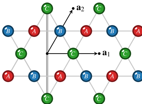
Figure 5: Kagome lattice with space group p6m . The A , B , and C sublattices are labeled in red, blue, and green, respectively, but the sites are identical. The generating mirror, which is chosen to send x \mapsto -x , is denoted by the double gray line. The lattice translation vectors, \mathbf{a}_1 and \mathbf{a}_2 , are denoted by the black arrows.
