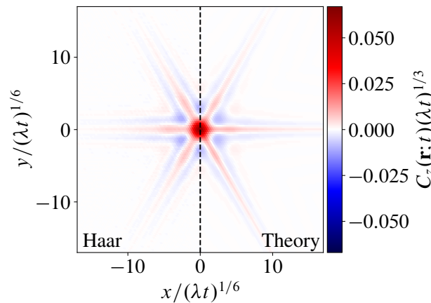
Figure 9: Comparison between the charge density autocorrelation function C_z(\mathbf{r}; t) = \langle \hat{S}^z(\mathbf{r}; t) \hat{S}^z(\mathbf{0}; 0) \rangle obtained for a Haar-random circuit that conserves the multipole moments (33) (left) and the corresponding hydrodynamic prediction (38) (right). The correlation function is evaluated using an effective classical automaton evolution that allows us to reach large systems and times. The spatial profile is illustrated at a fixed time, t = 5 \times 10^3 , for a system of linear size L = 512 .
