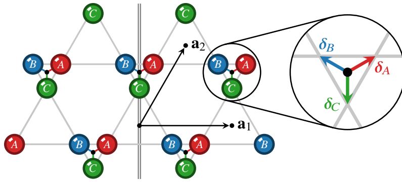
Figure 8: Breathing Kagome lattice, which belongs to the space group p3m1 . The A , B , and C sublattices are labeled in red, blue, and green, respectively, but the sites are identical. The generating mirror, which is chosen to send x \mapsto -x , is denoted by the double gray line. The lattice translation vectors, \mathbf{a}_1 and \mathbf{a}_2 , are denoted by the black arrows. The C_3 rotation center to which each basis site is associated is depicted by a solid black circle. The zoomed circular inset illustrates the three vectors \delta_i that connect Bravais sites to basis sites.
