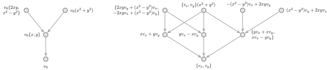
Figure 6: Mixing of irreps by translational symmetry for the Kagome (and breathing Kagome) lattice(s). Every arrow means that some (infinitesimal) translation acting on the polynomial(s) of higher degree generates the polynomial(s) of lower degree. Unlike previous trees, there exist two disjoint hierarchical structures. Physically, this means that there exist valid multipole groups that do not include total charge. The shorthand notation v_0 = (1, 1, 1)^T , v_x = \frac{1}{2}(\sqrt{3}, -\sqrt{3}, 0)^T , and v_y = \frac{1}{2}(-1, -1, 2)^T is used for the vectors that span the three-dimensional space that corresponds to the sublattice index. The representations of the polynomials under the point group are given in Table 3.
