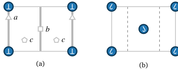
Figure 7: Left: An example of a lattice belonging to the space group pm . Axes of reflection are denoted by the double gray lines. The labels a , b , and c correspond to the three types of Wyckoff position, with multiplicities one, one, and two, respectively. Right: A lattice with space group pg . The dashed gray lines represent axes of glide reflection since the two types of lattice site are (only) mapped onto one another under the mirror x \mapsto -x (supposing they were spatially coincident). The solid gray lines represent lattice translations, which are parallel to the x - and y -axes.
