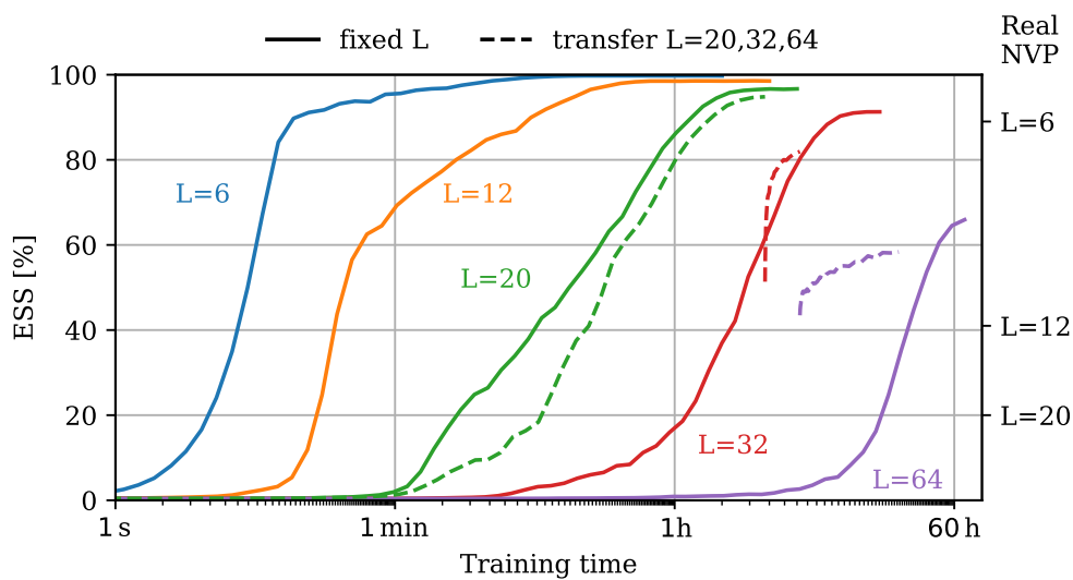
Figure 1: The effective sample sizes for lattice sizes L \times L of our model with coupling constants as in Table 1. Dashed lines show the result of transfer learning from L = 20 to L = 64 with fixed coupling \lambda = 4.398 . Ticks on the right indicate the ESS values 89%, 44%, 8.3%, 1.4% achieved with the real NVP architecture for lattice sizes L = 6, 12, 20, 32 with coupling constants as in Table 1.
