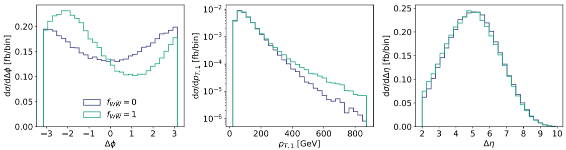
Figure 9: Kinematic distributions for WBF Higgs production at parton level with different Wilson coefficients f_{W\widetilde{W}} . Here, \Delta\phi denotes the signed azimuthal angle between the two tagging jets, p_{T,1} refers to the leading tagging jet, and \Delta\eta = |\Delta\eta_{jj}| .
