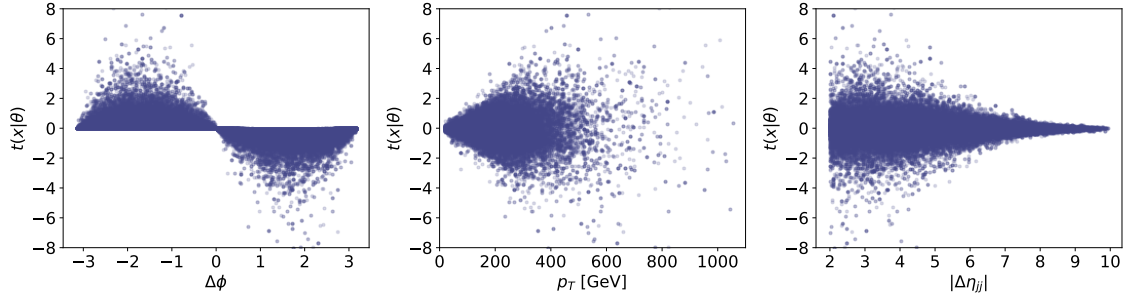
Figure 10: Score for simplified WBF Higgs production at parton level and with f_{W\widetilde{W}} = 0 .
