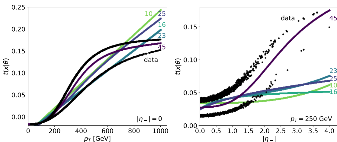
Figure 8: Sliced kinematic distributions for the complete ZH setup with f_B = 10 , showing the HoF given in Tab. 7.
