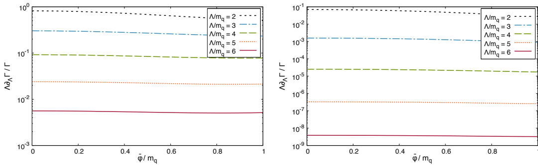
Figure 2: Change of the effective action at \bar{\Delta} = 0 under a variation of the UV scale \Lambda , i.e. \Lambda \partial_\Lambda \Gamma , relative to the effective action \Gamma itself as a function of \bar{\varphi} for T/m_q = 1/2 and \mu = 0 (left panel) as well as for T/m_q = 1/5 and \mu/m_q = 1 (right panel) for various different values of \Lambda/m_q , where m_q \approx 0.300 GeV is the vacuum quark mass.
