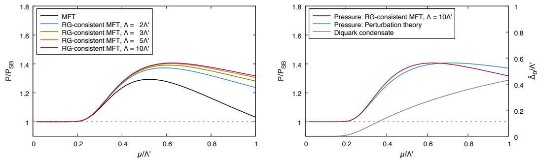
Figure 1: Left panel: Pressure P/P_{SB} of our diquark model as a function of the chemical potential \mu/\Lambda' (with \Lambda' = 0.6 \text{ GeV} ) as obtained from conventional mean-field theory (MFT) with a UV cutoff \Lambda = \Lambda' (black line) as well as from RG-consistent MFT with \Lambda/\Lambda' = 2, 3, 5, 10 . Right panel: Pressure P/P_{SB} of our diquark model as a function of the chemical potential \mu/\Lambda' as obtained from RG-consistent MFT with \Lambda/\Lambda' = 10 together with the perturbative expression for the pressure at leading order in the weak-coupling expansion, see Eq. (46). Moreover, we also show the gap \bar{\Delta}_0/\Lambda' (gray line) as extracted from RG-consistent MFT with \Lambda/\Lambda' = 10 .
