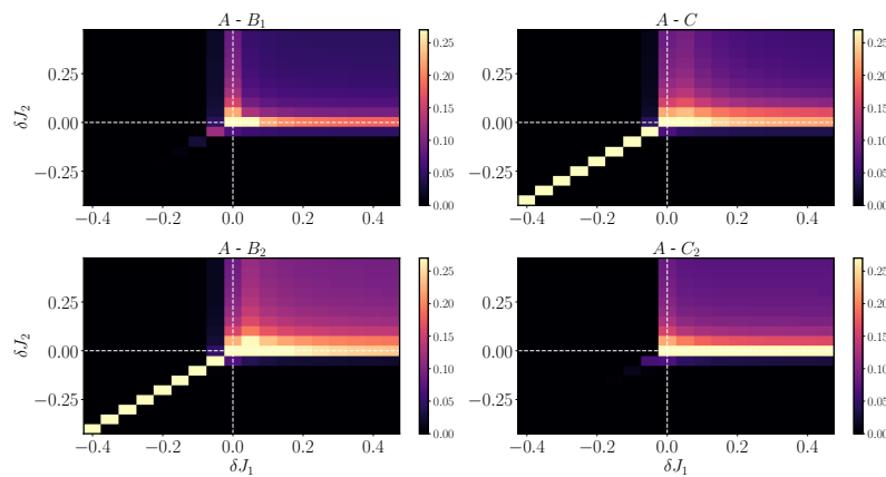
Figure 11: Density plot of the disconnected Renyi-2 entropy computed for the AFM Ising chain ( J = 1 ) with two bond defects and transverse magnetic field h = 0.5 for a chain with N = 121 spins. The \delta J_1 defect is in the A subpartition. White dashed lines guide the eye and indicate where each defect turns from favoring a ferromagnetic alignment on that bond to an AFM one.
