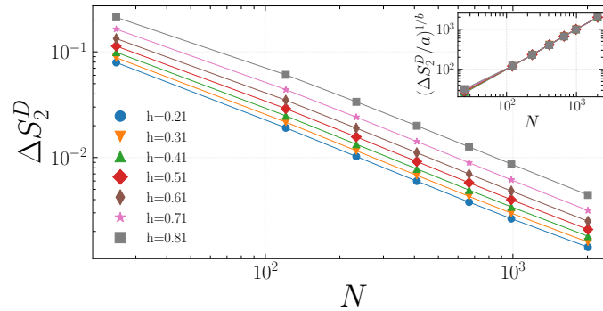
Figure 4: Behavior of \Delta S_2^D(N) in eq. (12) as a function of the chain length N . We observe that in the thermodynamic limit, regardless of the value of h , it vanishes with the law \Delta S_2^D = aN^b with b \simeq -0.935 \pm 0.006 . In the inset, we provide the proof of the generality of the dependence of \Delta S_2^D(N) on N , showing the scaling relation (\Delta S_2^D / a)^{(1/b)} = N .
