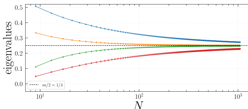
Figure 8: Non-vanishing eigenvalues of the reduced density matrix in eq. (17) as a function of the size of the chain for M = mN = (N - 1)/2 . In this case, in the thermodynamic limit, all the eigenvalues tend to 1/4 .
