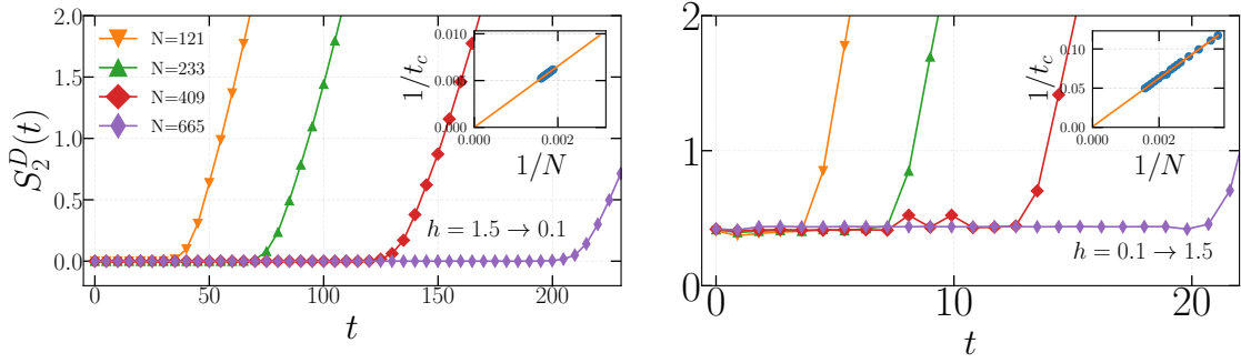
Figure 5: Time evolution of the disconnected Rényi-2 entropy after a global quantum quench. Left panel S_2^D after quenching the Hamiltonian from the paramagnetic phase ( h = 1.5 ) to the frustrated one h = 0.1 as a function of time and for different system sizes N . Right panel S_2^D after quenching the Hamiltonian from the frustrated phase h = 0.1 to the unfrustrated one h = 1.5 as a function of time and for different system sizes N . In both cases, S_2^D after the quench remains constant up to a critical time t_c that depends on the size of the system and diverges with N . This is shown in the insets where the inverse critical time 1/t_c is plotted against the inverse chain length 1/N and one sees that a linear extrapolation shows divergence of t_c as N \rightarrow \infty . In all these simulations, we used m = (N - 1)/2N \approx 1/2 , and l = (N - 1)/8N \approx 1/8 .
