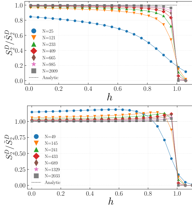
Figure 3: Disconnected Renyi-2 entanglement entropy as a function of the magnetic field h for different lengths of the system. Upper panel: we fix the dimension of the subpartition to m = \frac{N-1}{2N} \approx \frac{1}{2} and l = \frac{N-1}{8N} \approx \frac{1}{8} . Bottom panel: we chose m = \frac{N-1}{4N} \approx \frac{1}{4} and l = \frac{5(N-1)}{16N} \approx \frac{5}{16} . We normalize S_2^D by its quantization value \tilde{S}_2^D(m, l) in eq. (9) and draw in black a horizontal line at S_2^D / \tilde{S}_2^D = 1 to guide the eye toward the asymptotic value. We observe that in the frustrated phase ( h < 1 ), there is long-range entanglement in accordance with our theory and that it drops to zero for h > 1 .
