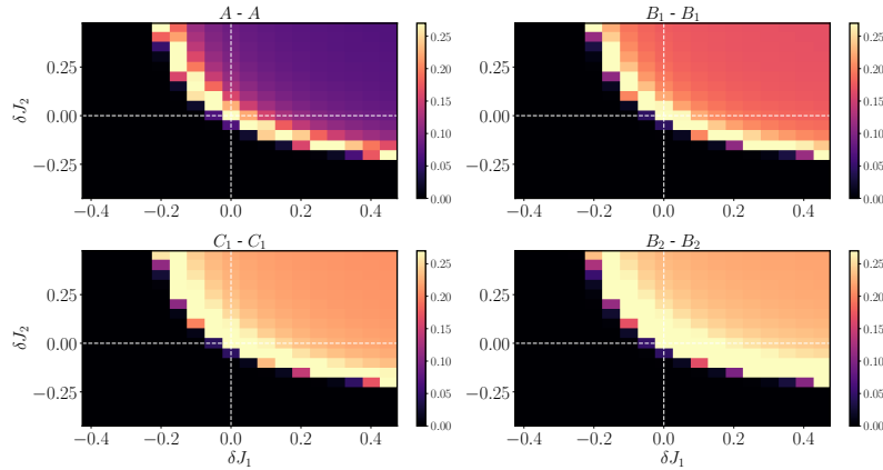
Figure 14: Density plot of the disconnected Renyi-2 entropy computed for the AFM Ising chain ( J = 1 ) with two bond defects placed in the middle of the same subpartition at neighbor sites, and transverse magnetic field h = 0.5 . White dashed lines guide the eye and indicate where each defect turns from favoring a ferromagnetic alignment on that bond to an AFM one. The DEE is non-zero even in the presence of one ferromagnetic defect, provided that the neighboring one is anti-ferromagnetic and enough strong.
