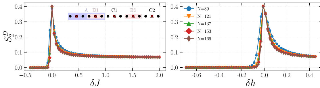
Figure 6: Left : Renyi-2 disconnected entanglement entropy S_2^D as a function of the bond disorder strength \delta J for \delta h = 0 Right : Renyi-2 disconnected entanglement entropy S_2^D as a function of the field disorder strength \delta h for \delta J = 0 In both cases, we have assumed J = 1 and h = 0.5 while we have placed the defect in the center of the A/B1 subsystem.
