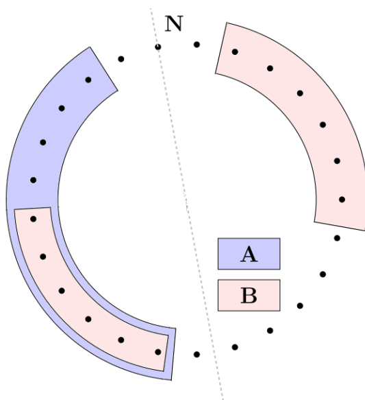
Figure 1: Sketch of the subsystems used in the disconnected Renyi- \alpha entanglement entropy in Eq. (5). The black dots represent the spins in the chain ( N is always chosen to be odd). For what concern the subsystems, one of the two parts of B is always included in A , while the other is a subset of A^c . Moreover, the subset A and the part of B included in it always share a boundary.
