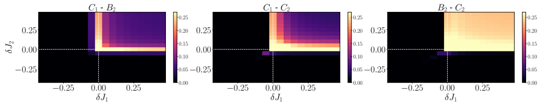
Figure 13: Density plot of the disconnected Renyi-2 entropy computed for the AFM Ising chain ( J = 1 ) with two bond defects and transverse magnetic field h = 0.5 for a chain made of N = 121 spins. The \delta J_1 defect is in the C_1 subpartition (first two panels from the left) and in the B_2 ones (last panel from the left). White dashed lines guide the eye and indicate where each defect turns from favoring a ferromagnetic alignment on that bond to an AFM one. We observe a non-zero DEE when both defects favor an antiferromagnetic alignment ( \delta J_1, \delta J_2 > 0 ).
