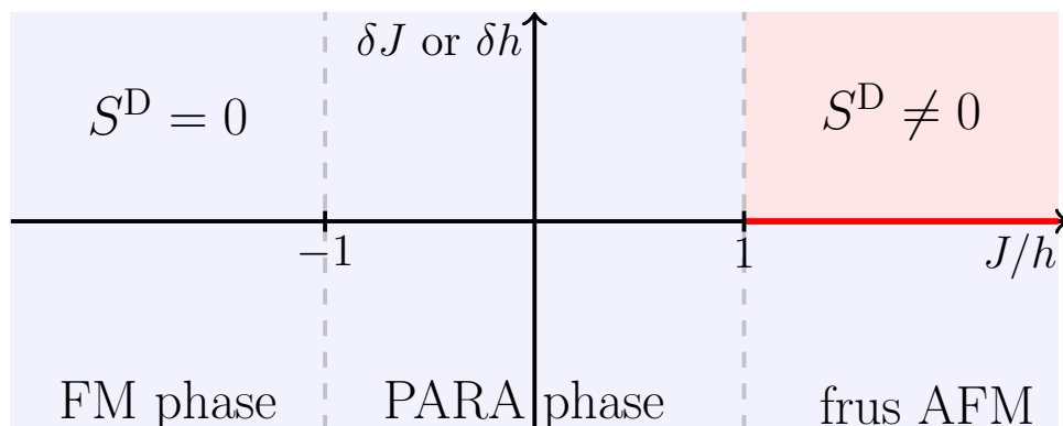
Figure 7: Phase diagram of the geometrically frustrated Ising spin chain in Eq. (14) with respect to a single bond or site disorder \delta J and \delta h , respectively. The disconnected entanglement entropy S^D shows a non-vanishing value (red color) in the thermodynamic limit (TD) for positive disorder strengths. Additionally, the red line denotes where the exact results are obtained. See Sec. 2 and Eq. 14 for more details about considered model.
