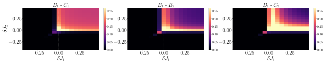
Figure 12: Density plot of the disconnected Renyi-2 entropy computed for the AFM Ising chain ( J = 1 ) with two bond defects and transverse magnetic field h = 0.5 for a chain with N = 121 spins. The \delta J_1 defect is in the B_1 subpartition. White dashed lines guide the eye and indicate where each defect turns from favoring a ferromagnetic alignment on that bond to an AFM one. We observe a non-zero DEE when both defects favor an antiferromagnetic alignment ( \delta J_1, \delta J_2 > 0 ).
