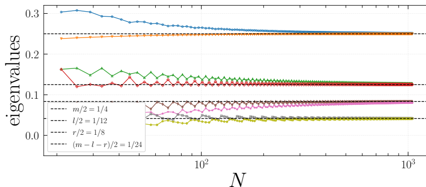
Figure 9: Non-vanishing eigenvalues of the reduced density matrix in eq. (19) as a function of the size of the chain for M = mN = (N - 1)/2 , R = rN = (N - 1)/4 , and L = lN = (N - 1)/6 . In this case, in the thermodynamic limit, two eigenvalues admit as limit 1/4 and two of the other six tend to 1/8 . Of the last four, two tend towards 1/12 , and the last two admit as their limit 1/24 .
