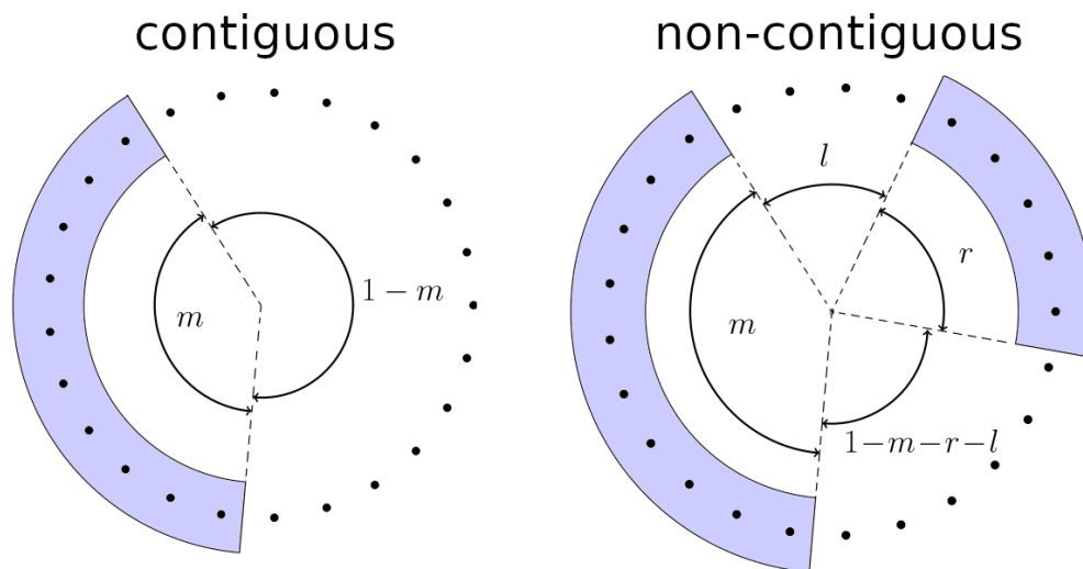
Figure 2: Generic partitions considered in respect to Eq. (5). We consider a contiguous subset of m = M/N spins in the left panel while, in the right one, the subsystem of interest is divided into disconnected sectors of length m = M/N and r = R/N , while being separated by l = L/N spins.
