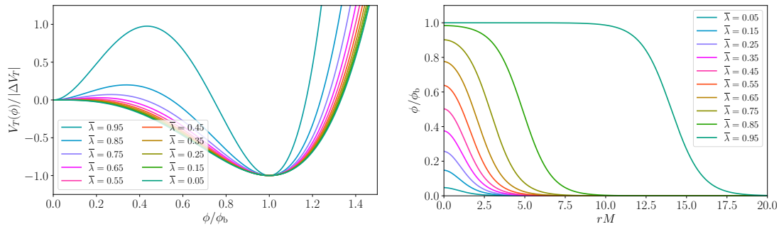
Figure 9: Left panel: the scaled quartic potential as a function of the parameter \bar{\lambda} , defined in Eq. (6.18). Right panel: the critical bubble solution to Eq. (6.17). Scripts by kind permission of D. Cutting, see also Ref. [55].
