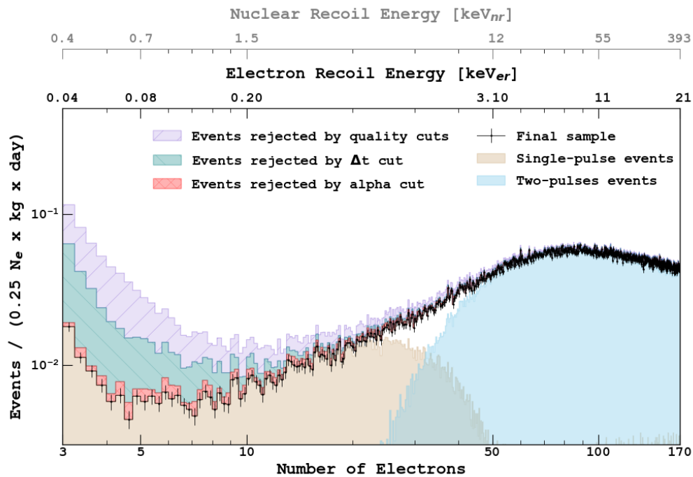
Figure 1: Observed electron spectra at different steps of the event selection.
