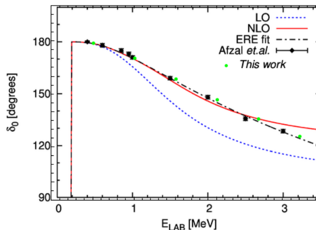
Figure 2: \alpha\alpha scattering phase shift \delta_0 ( l = 0, j = 0 ) with cutoff \Lambda = 100\text{ MeV} in comparison with experimental data from Afzal et al. [15] and with another Halo EFT calculation [7] in lowest order (LO) and Next-to-leading order (NLO). Also shown their fit using the effective range expansion formula (ERE fit).
