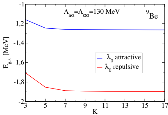
Figure 3: Convergence of {}^9\text{Be} ground state energy as a function of the HH quantum number K with \Lambda_{\alpha n} = \Lambda_{\alpha\alpha} = 130 MeV.
