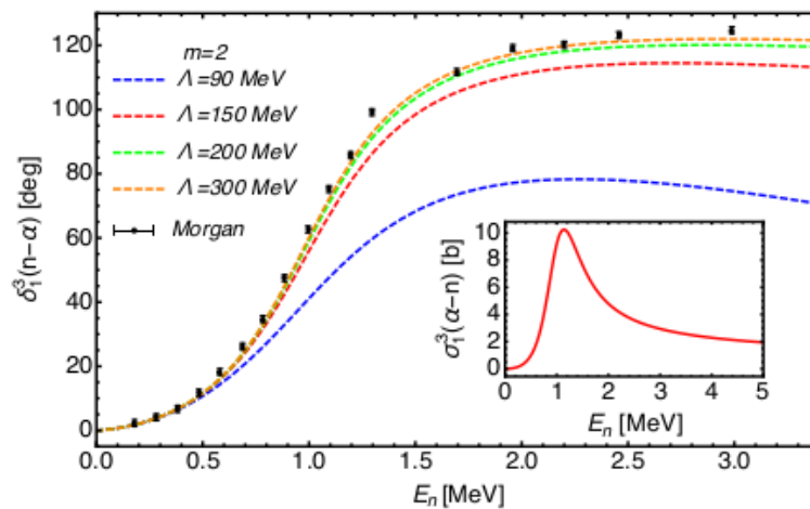
Figure 1: Phase shifts \delta_{13}(E_n) ( l = 1, J = 3/2 ) with experimental data from Morgan and Walter [14] and in the inset the cross-section \sigma_{13}(E_n) obtained with \Lambda = 300\text{MeV} .
