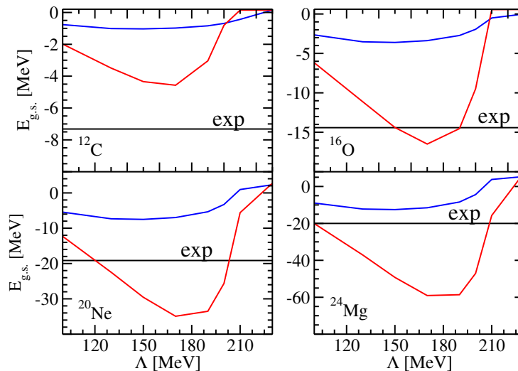
Figure 6: Cutoff dependence of ground-state energies of various \alpha -nuclei with HH quantum number K equal to 12 ( {}^{12}\text{C} , {}^{16}\text{O} ) and 8 ( {}^{20}\text{Ne} , {}^{24}\text{Mg} ). Blue curves: \lambda_0 attractive; red curves: \lambda_0 repulsive.
