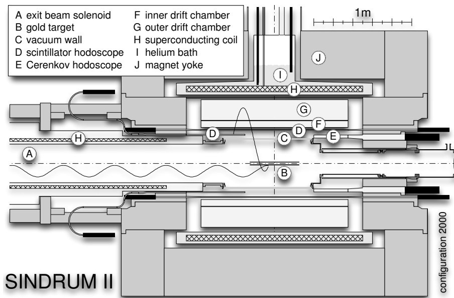
Figure 8.1: The SINDRUM II spectrometer as configured in the year 2000.
