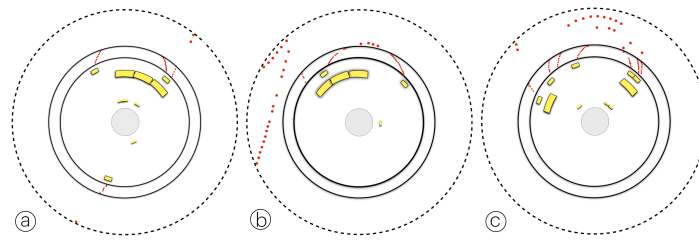
Figure 8.6: Three cosmic-ray events in the r\phi projection. Signals recorded in the drift chambers (red), the plastic hodoscopes and Čerenkov counters (yellow) are indicated: a) a high momentum muon knocking an e^- out of a Čerenkov counter, b) a high momentum muon creating an e^+e^- pair in the magnet coil and c) an e^+ (most likely from the decay of a distant cosmic muon) spiraling in from outside.
