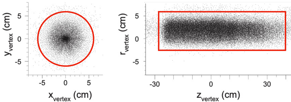
Figure 8.8: Reconstructed point of closest approach to the z axis in the xy and zr projections. The contours indicate the selected target region.
