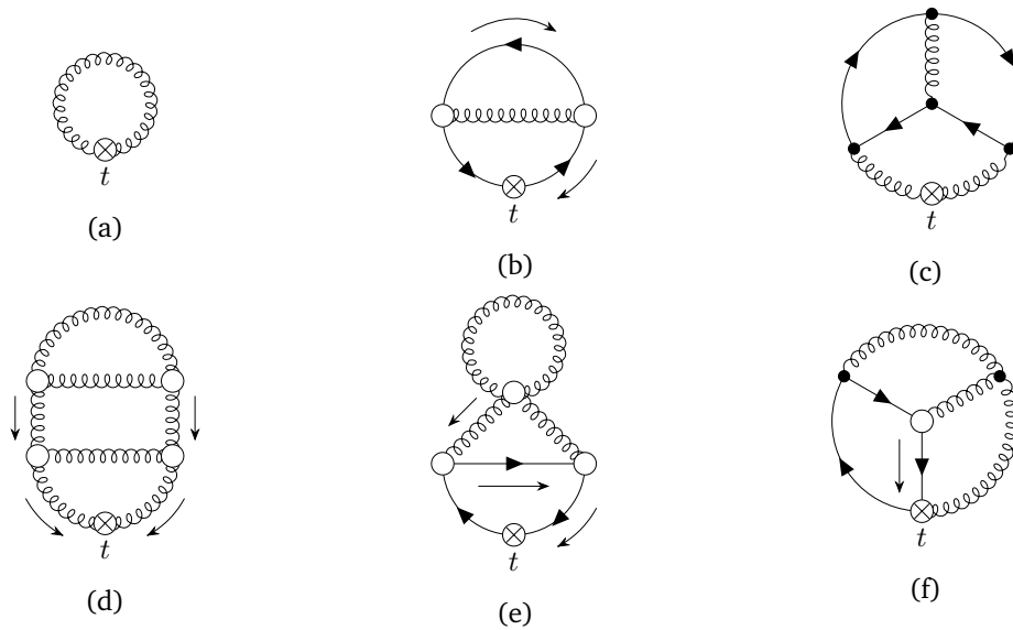
Figure 1: Sample diagrams for the VEVs through NNLO. Produced with TikZ-Feynman [16].
