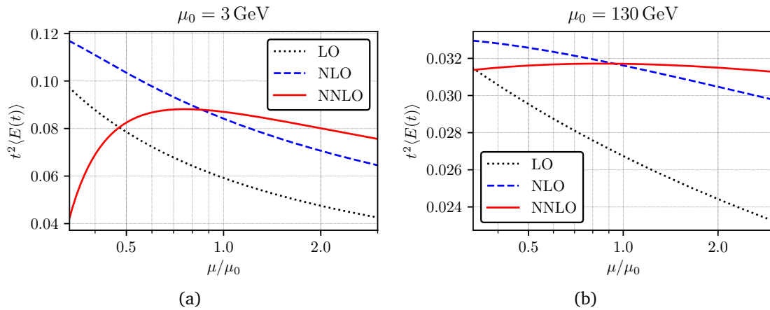
Figure 2: Renormalization scale dependence of t^2 \langle E(t) \rangle in QCD for two different central scales \mu_0 = e^{-\gamma_E/2}/\sqrt{2t} . See Ref. [13] for details.
