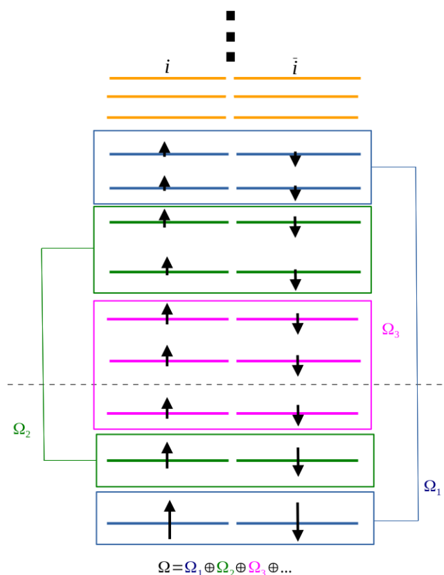
Figure 1: Partition of the spinor space \Omega into subspaces mutually disjoint \Omega_p . While arrows refer to \alpha or \beta spin in the nonrelativistic context, in this work they correspond to electrons occupying spinors that are Kramers' pairs. Let us remark that some NOs may remain uncoupled (a.k.a. virtual spinors) like the orange ones in this scheme.
