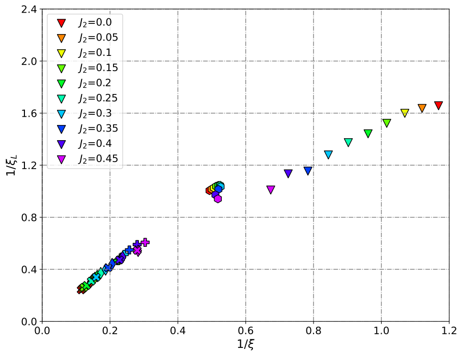
Figure 7: Longitudinal correlation length \xi_L , as extracted from the spin-spin correlations, as a function of the transverse one \xi for different values of J_2/J_1 at D = 3, \dots, 7 (denoted by triangles, hexagons, pluses, diamonds, and crosses in the same order).
