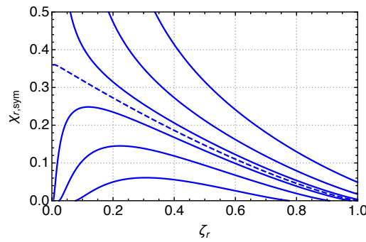
Figure 1: The classical field \hat{\chi}_{r,\text{sym}} as a function of the gauge parameter \zeta_r for increasing (top to bottom) values of \beta_r/\bar{g}_r^2 (in units of \bar{\mu}^2 ). The dashed curve is the case \beta_r/\bar{g}_r^2 = 0 . For positive values of this parameter (curves below the dashed one), solutions of the gap equation (22) with \hat{\chi}_{r,\text{sym}} \geq 0 only exist in a range of parameters limited by the inequalities (23).
