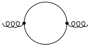
Figure 3: The loop contribution from the N_k^\alpha superfields to the gluon two-point vertex function.
