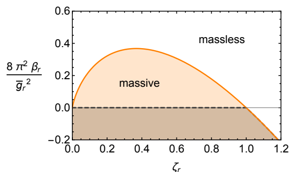
Figure 2: The phase diagram of the theory in terms of the parameters \beta_r/\bar{g}_r^2 and \zeta_r (in units of \bar{\mu}^2 ). The orange line separates the phase of broken symmetry (white region), where there is no generation of a gluon mass at tree level, from that of restored symmetry (shaded region), with \hat{N}^\alpha = 0 , where a nonzero gluon mass is generated at tree level. The transition between the two phases is continuous. In the massive phase, the renormalized tree-level square gluon mass is \beta_r . The shaded region with \beta_r < 0 is thus excluded in a perturbative setting.
