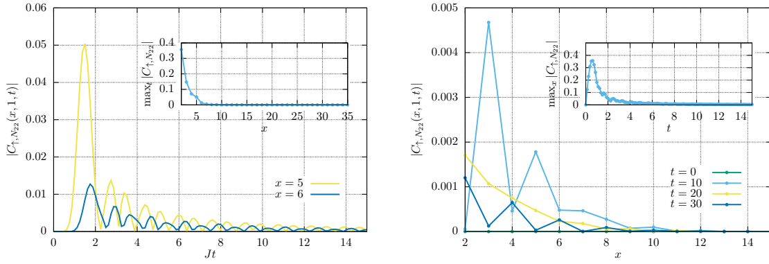
Figure 4: Dynamics of the bulk boundary correlation C_{\uparrow, N_{22}}(x, 1, t) after a quench from the nested Néel state (119) in the thermodynamic limit. The left panel reports the time evolution of |C_{\uparrow, N_{22}}(x, 1, t)| at two specific positions while the right panel shows four fixed-time cuts of |C_{\uparrow, N_{22}}(x, 1, t)| (the insets respectively show the decay in x of \max_t |C_{\uparrow, N_{22}}(x, 1, t)| and in t of \max_x |C_{\uparrow, N_{22}}(x, 1, t)| ).
