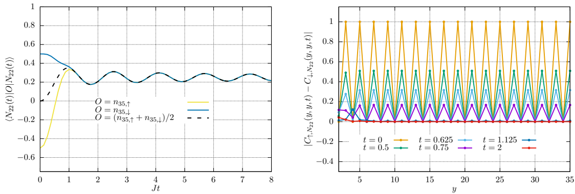
Figure 3: Dynamics of the number operators after a quench from the generalised nested Néel state (119) in the thermodynamic limit. The left panel shows the time evolution of the densities at x = 35 , comparing C_{\uparrow, N_{22}}(y, y, t) , C_{\downarrow, N_{22}}(y, y, t) , and (C_{\uparrow, N_{22}}(y, y, t) + C_{\downarrow, N_{22}}(y, y, t))/2 = \langle N_f | d_y(t) | N_f \rangle / 2 . The right panel shows fixed-time slices of |C_{\uparrow, N_{22}}(y, y, t) - C_{\downarrow, N_{22}}(y, y, t)| .
