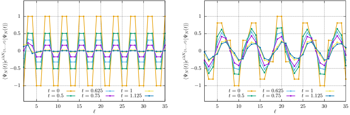
Figure 2: Characteristic function \chi_N(t, A, \lambda) (cf. (67)) vs subsystem size for different times after a quench from the state (60) in the thermodynamic limit. The two panels correspond to \lambda = \pi (left) and \lambda = 7\pi/5 (right). In both cases \chi_N(t, A, \lambda) approaches 0 for all \ell for large times, signalling the melting of the order.
