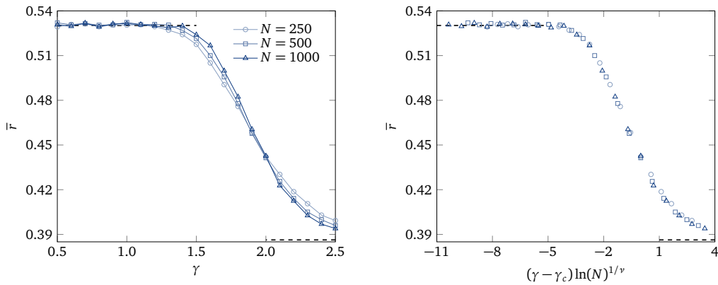
Figure 1: The average ratio of consecutive level spacing spacings \bar{r} as a function of \gamma (left panel) and (\gamma - \gamma_c)\ln(N)^{1/\nu} with \gamma_c = 2 and \nu = 1 (right panel) for matrix dimensions N = 250, 500, and 1000 . Poissonian and Wigner-Dyson level statistics are characterized by respectively \bar{r} \approx 0.386 and \bar{r} \approx 0.530 (dashed lines).
