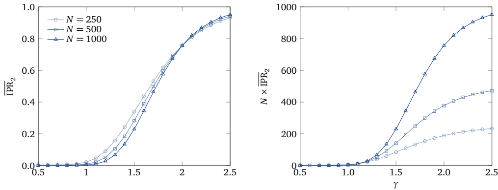
Figure 2: The average of the inverse participation ratio \overline{IPR_2} (left panel) and the value scaled by N (right panel) as a function of \gamma for matrix dimensions N = 250, 500, and 1000 .
