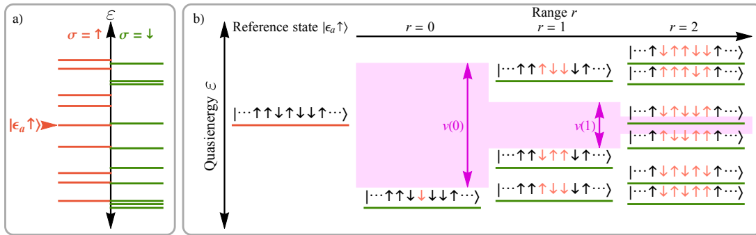
Figure 4: Organising resonances by range: a) The many-body spectrum of \mathcal{H}_0 in a small quasi-energy window is divided into two sectors labelled by the state of the probe spin \sigma = \uparrow, \downarrow . |\epsilon_a \uparrow\rangle labels a specific reference state. b) The l-bit configuration corresponding to reference state (red spectral line) is shown. The states |\epsilon_d \downarrow\rangle in the opposite sector (green lines) can be grouped according to their range r from the reference state (ranges r = 0, 1, 2 shown); states at range r differ only on the l-bits with index |n| \leq r (highlighted in orange). A state |\epsilon_d \downarrow\rangle at range r is resonant with |\epsilon_a \uparrow\rangle if its quasi-energy separation is less than the matrix element size v(r) (i.e. if it lies within the magenta region). In the plot, the first resonance occurs at range r = 2 .
