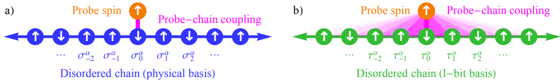
Figure 3: Set-up in the physical and l-bit bases respectively: a) A “probe” spin- \frac{1}{2} (orange) couples to a strongly disordered chain (blue) at the site n = 0 (magenta). b) Transforming to the l-bit basis renders the Floquet unitary of the chain diagonal and the probe-chain coupling quasi-local. The coupling strength decays exponentially with distance from n = 0 .
