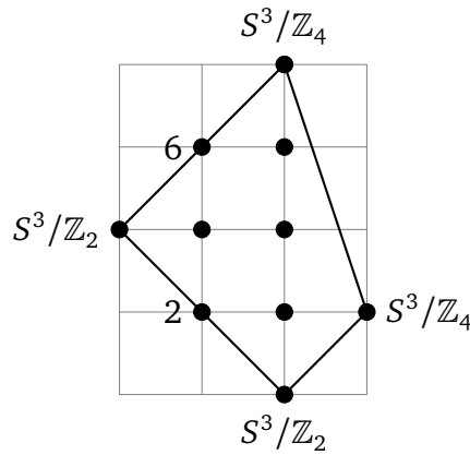
Figure 6: The toric diagram for SU(2)_0 - SU(4)_0 quiver.
