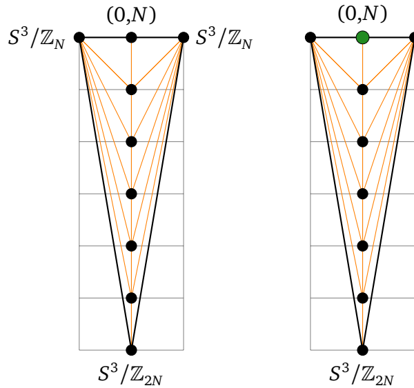
Figure 5: The toric diagram from SU(N)_N shown here on the left for SU(6)_6 , which has \mathbb{Z}_6 1-form symmetry. The orange lines indicate the triangles which determine the order of the S^3/\mathbb{Z}_k quotient. The right figure shows the toric diagram after we excise the A_1 singularity (shown in green), which is associate to the \mathcal{F} = SO(3) flavor symmetry group. The only remaining lens space is the S^3/\mathbb{Z}_{2N} . For even N this forms a non-trivial extension with the 1-form symmetry \mathbb{Z}_N and thereby a 2-group.
