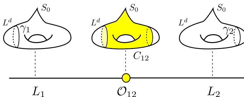
Figure 1: The geometric description of a line changing operator \mathcal{O}_{12} connecting line operators L_1 and L_2 as a chain (shown in yellow) connecting homologous cycles on the boundary.
