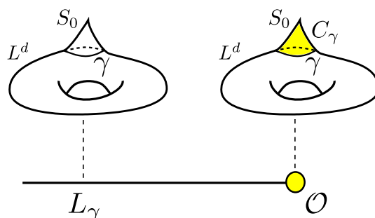
Figure 2: A line operator associated to a homologically trivial curve \gamma on L^d ending on a point operator. From the point of view of the internal geometry L^d the point operator at the end corresponds to the M2-brane worldvolume wrapping a chain C_\gamma with boundary \gamma .
