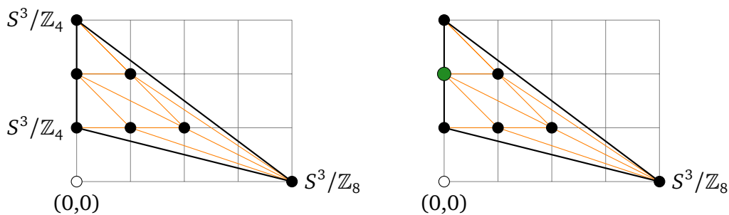
Figure 7: The toric diagram from B_4^{(2)} .
