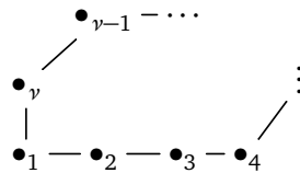
Figure 3: Schematic topology of \mathbb{C}^3_{L_{\mathcal{X}}} [63] – see also [26] for the case \mathcal{X} non-isolated. In this figure we have 4 vertices along an external edge corresponding to a \mathbb{C}^2/\mathbb{Z}_3 singularity. We denote as \mathcal{S} the neighborhood of the singular locus we need excise when considering the 2-group structure – clearly after the excision the Lens spaces L_1 and L_4 in the above figure become contractible and do not contribute to H_1(L_{\mathcal{X}}^5 - \mathcal{S}) .
