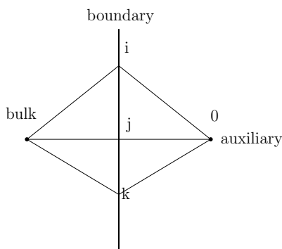
Figure 3: Auxiliary simplices connected to auxiliary vertex 0.
