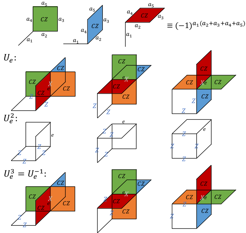
Figure 5: The operator U_e on the cubic lattice.
