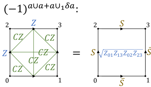
Figure 14: “Electric” string operator.
