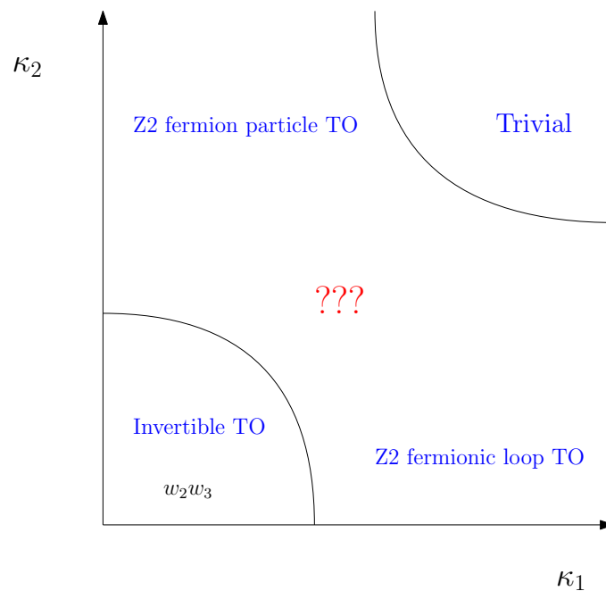
Figure 9: Sketch of the phase diagram of the Hamiltonian model (70) in (4+1)D. The phase transition(s) along the 45 degree line \kappa_1 = \kappa_2 are protected by the non-trivial invertible topological order on the lower left corner. The \mathbb{Z}_2 fermionic loop topological order in (4+1)D has three non-trivial basic excitations: electric loop, magnetic loop, and dyonic loop, where the magnetic and dyonic loop excitations are fermionic while the electric loop excitation is bosonic (similar theory with only bosonic loop excitations is discussed in Ref. [53]).
