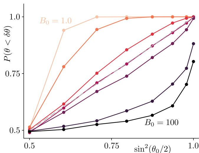
Figure 2: Reproducing Born’s rule. The relative frequency of evolutions coming within \delta\theta of the state |0\rangle is plotted as a function of the initial weight \sin^2(\theta_0/2) . Dots represent calculated values, while lines are included as a guide to the eye only. The diagonal dashed line indicates Born’s rule, while the differently coloured data sets show different values of the parameter B_0 , ranging from B_0 = 1.0 at the top through 2.0, 5.0, 7.0, 10, 50, and B_0 = 100 at the bottom. We set J = 1 throughout. For each set of parameter values, 10^4 instances of the dynamics are calculated for a maximum of 20^3 time steps. Taking \tau_r small compared to \tau_c and the size of time steps, the random variable \chi \in [0, \pi] is sampled each time step from the probability density function \sin(\chi)/2 , which yields a flat distribution for the value of \cos(\chi) .
