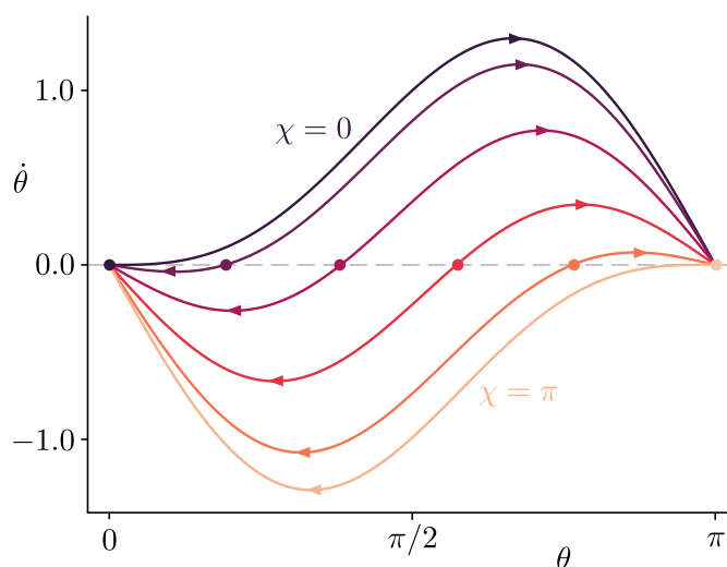
Figure 1: Flow diagram for the pointer state dynamics. The rate of change \dot{\theta} is depicted as a function of the instantaneous angle \theta for different values of the random variable \chi , ranging from \chi = 0 (dark, top) to \chi = \pi (light, bottom). Here, we used J = B_0 . The arrows show the direction of flow, while the dots indicate fixed points.
