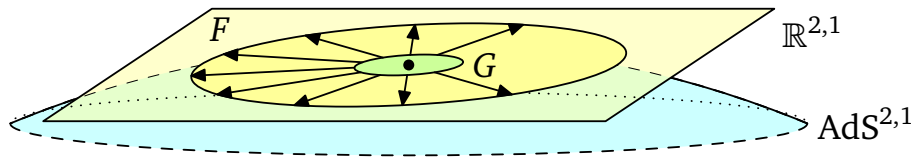
Figure 1: Mapping between a function on a small neighbourhood of a point on \text{AdS}^{2,1} and a function on the tangent space.
