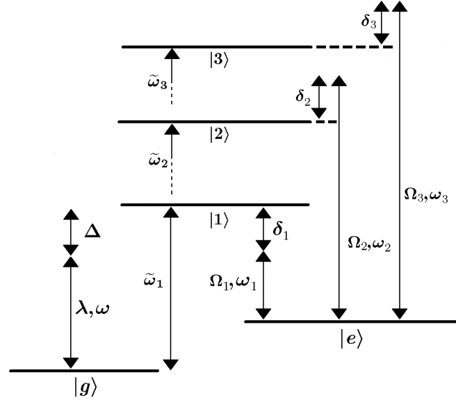
Figure 2: Atomic configuration to engineer the non-Hermitian Jaynes-Cummings interaction.
