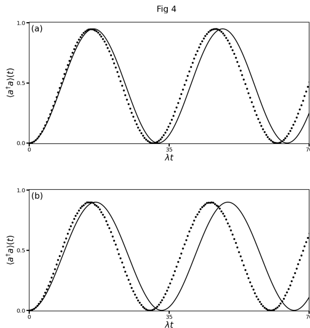
Figure 4: Plot of \langle a^\dagger a \rangle(t) against |\lambda|t computed from the full Hamiltonian (15) (dotted line) and the effective one (16) (solid line), for R = 0.95 , and 0.9 , considering \alpha = 0.1 and \Delta_2 = \Delta_3 = 5 \times 10^3 \lambda for all values of R . For R = 0.95 we fixed (in units of \lambda ) \beta = 9.5 \times 10^{-2} , |\Omega_1| = 9.3 , |\Omega_2| = |\Omega_3| = 120 , \Delta = 92.6 and \Delta_1 = 97.5 . For R = 0.9 we fixed \beta = 9 \times 10^{-2} , |\Omega_1| = 6.6 , |\Omega_2| = |\Omega_3| = 141.2 , \Delta = 66.4 and \Delta_1 = 73.8 .
