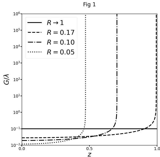
Figure 1: Plot of G/\lambda against z for R = 1.0, 0.17, 0.1 and 0.05 , as indicated by solid, dashed, dashed-dotted and dotted lines, respectively, assuming \alpha = 10^{-1} > \beta .
