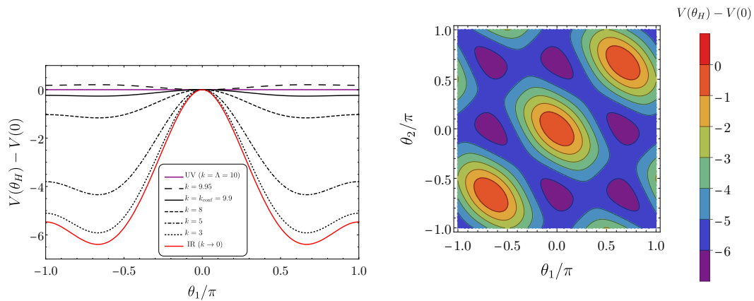
Figure 8: The potential with m_{\text{gap}}^2 = 10^2 and k_{\text{conf}} = 9.9 in a confinement-emulated scenario. Left: The renormalization evolution of the potential at the \theta_2 = 0 plane from \Lambda = 10 to k = 0 . Right: Contour plot of the potential at the IR scale k \rightarrow 0 in \theta_1 - \theta_2 plane.
