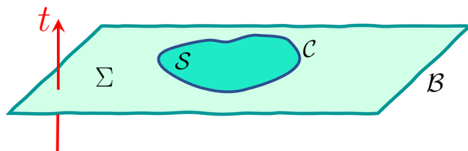
Figure 1: \Sigma is a constant time slice, a Cauchy surface, B is its boundary. S is a generic section of \Sigma and C is its boundary.
