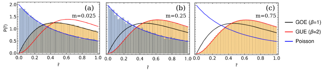
Figure 9: Level spacing ratio distribution P(\tilde{r}) in both sectors (RMT and Poisson) for m = 0.025 (a), m = 0.25 (b) and m = 0.75 (c), in the limit g \rightarrow \infty . In panel (c), there is just one histogram, because for m > 0.5 only the RMT sector is present. The histograms related to the RMT sectors (in yellow) were obtained by exact diagonalization of Eq. (46) for N_F = 3000 and 1000 different realizations. The histograms related to the Poisson sector (in blue) were obtained by solving Eq. 47) for N_F = 500 and 100 distinct realizations. The colored lines correspond to the analytical results of Eqs. (57) and (58). We find perfect agreement with the theoretical predictions in each case.
