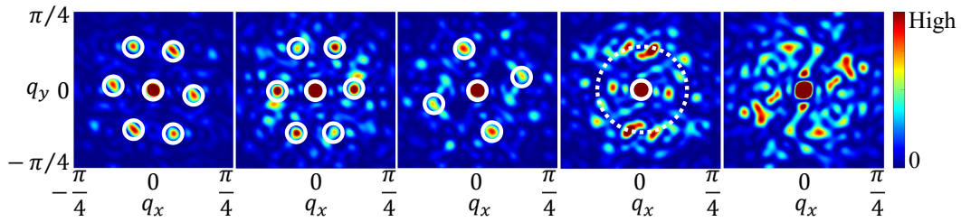
Figure 5: Structure factor of the position of vortices in the weak disorder region V = 0.5 . The magnetic flux is \phi/\phi_0 is 16, 18, 20, 22 and 24 from left to right. For \phi/\phi_0 = 16, 18 , the pattern is consistent with a triangular lattice in real space. However, a small increase, \phi/\phi_0 = 20 , leads to a transition to a rectangular lattice. An increase in the flux ( \phi/\phi_0 = 22 ) results in a close to circular pattern signaling the absence of translational symmetry. Physically, a circular pattern indicates a combination of vortices repulsion and the restoration of rotational symmetry [65, 76]. This circular pattern eventually disappears for \phi/\phi_0 \geq 24 which signals a fully disordered phase with no clear vortex repulsion. To make the pattern more evident, we have set some cut-off value, referred by High in the plot.
