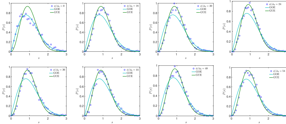
Figure 27: The level spacing distribution P(s) for V = 0.5 and different external magnetic flux is 0, 16, 20, 24, 36, 44, 48 and 54. The GOE is described by Eq (G.1), and GUE is Eq (G.2). The system size is N = 100 \times 100 , U = -1.25 and \langle n \rangle = 0.875 . For the statistical analysis, we only take 3000, 30% of the total, eigenenergies around the band center E = 0 . The observed good agreement with the random matrix prediction precludes any important effect of multifractality in this weakly disorder region.
