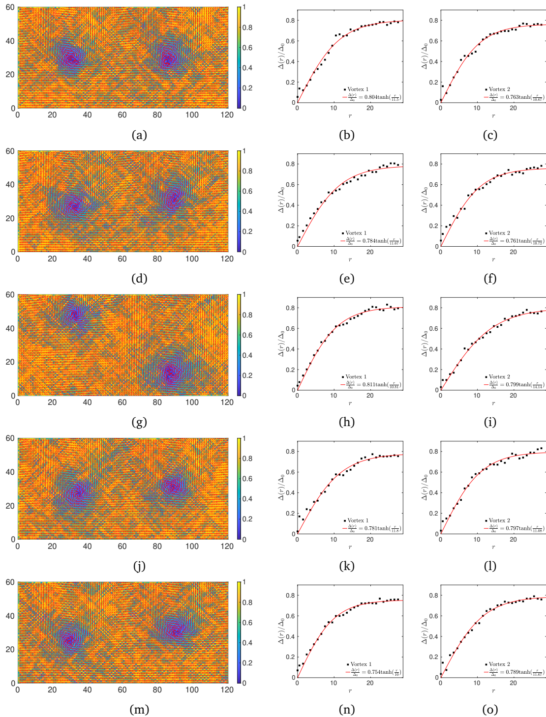
Figure 21: The spatial distribution of the order parameter and its phase in the weak disorder region V = 0.5 , and the corresponding vortex profile with the GL fit Eq. 4. Vortex 1 means the left vortex, and the right vortex is Vortex 2. Five different disorder realizations are presented. The other parameters are |U| = 1.0 , \langle n \rangle = 0.875 .
