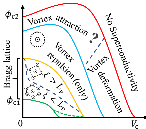
Figure 1: Vortex phase diagram. The cartoon summarizes the vortex distribution as a function of magnetic flux \phi and disorder V . The red (green) line stands for \phi_{c2} ( \phi_{c1} ) the upper (lower) critical magnetic flux as a function of the disorder strength V . In the region below the dashed green line, our results are not conclusive regarding the existence of a vortex lattice. Between the green and the sky blue line, we observe the expected Abrikosov triangular lattice. Upon increasing the magnetic flux, the lattice of vortices becomes rectangular when the average distance between vortices L_v is smaller than the superconducting coherence length \xi_0 . In the figure, we depict the Bragg lattice, the structure factor of the position of vortices. For larger fields, the circular pattern signals the vortex repulsion phase characterized by a loss of vortex translation symmetry, strong vortex repulsion and, on average, rotational symmetry of the position of vortices. In the phase termed vortex attraction, vortex repulsion is strongly suppressed and we observe strong vortex overlap in many cases. The question mark refers to the fact that we do not have a fully quantitative description of this phase. The phase termed vortex deformation is characterized by vortices with a vortex core that becomes spatially inhomogeneous and a highly deformed vortex profile. By no superconductivity, we refer to a region of vanishing superfluid density independently of its origin. We note that in the rest of regions, phase coherence holds. Indeed, disorder enhances the critical flux \phi_{c2} .
