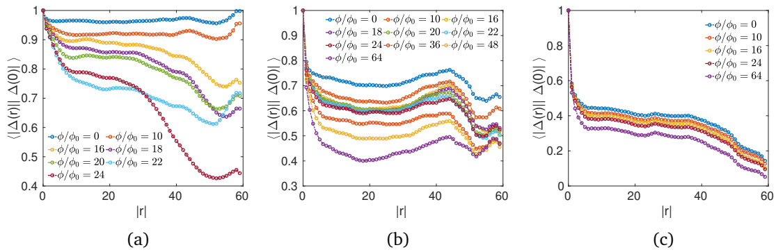
Figure 13: Two-point spatial correlation function of the order parameter. From left to right: V = 0.5, 1.5 and 2.25 . (a) The correlation is very sensitive to the magnetic flux strength. As a consequence, we observe substantial changes around the formation of the vortex lattice \phi/\phi_0 = 16 and its destruction \phi/\phi_0 = 22 . (b) The breaking of positional order is signaled by the insensitivity of the correlation function to changes in the field around \phi/\phi_0 \sim 20 . (c) Correlation function around the insulating transition. The dependence on the magnetic flux is rather weak in this region. Note the different range of fields in the left and right plots. The other parameters are |U| = 1.25, \langle n \rangle = 0.875 and the system size N = 60 \times 60 .
