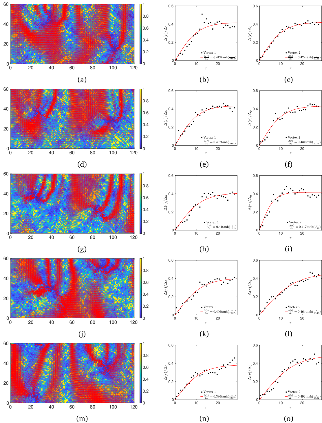
Figure 22: The spatial distribution of the order parameter and its phase in the intermediate disorder region V = 1.5 , and the corresponding vortex profile with GL fit. Vortex 1 means the left vortex, and the right vortex is Vortex 2. Five different disorder configurations are presented. The other parameters are |U| = 1.0 , \langle n \rangle = 0.875 .
