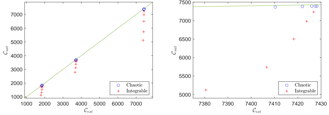
Figure 11: Left: The saturation height of the complexity bound against the estimate (53) for a few runs of the Ising model at L = 10, 11, 12 for k_{sp} = k_{op} = 2, 3, 4, 5, 6 for both the integrable case with (h_x, h_z) = (-1.05, 0) and the chaotic case (h_x, h_z) = (-1.05, 0.5) . The green line is C_{sat} = C_{est} . Right: We zoom in on the data for L = 12 .
