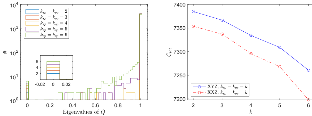
Figure 9: Left: The distribution of eigenvalues of the Q-matrix for the integrable XXZ model at (J_x = J_y, J_z) = (-0.35, -0.1) for increasing \mathcal{T}_1(k) , for L = 12 . In the bottom left corner, we zoom in on the number of exact zero eigenvalues. Right: A comparison between the late-time saturation values of the complexity bound as a function of \mathcal{T}_1(k) for the integrable XYZ at (J_x, J_y, J_z) = (-0.35, 0.5, -0.1) and XXZ model at (J_x = J_y, J_z) = (-0.35, -0.1) .
