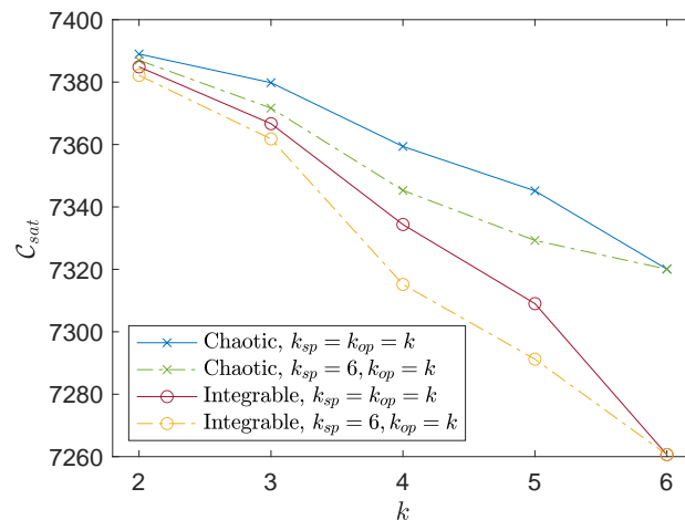
Figure 6: The late-time saturation value of the complexity bound for the integrable XYZ model (67) and the chaotic Hamiltonian with magnetic field (72) for L = 12 . For the coupling constants we used the numbers (J_x, J_y, J_z) = (-0.35, 0.5, -0.1) in both cases and h_z = 0.8 for the chaotic Hamiltonian.
