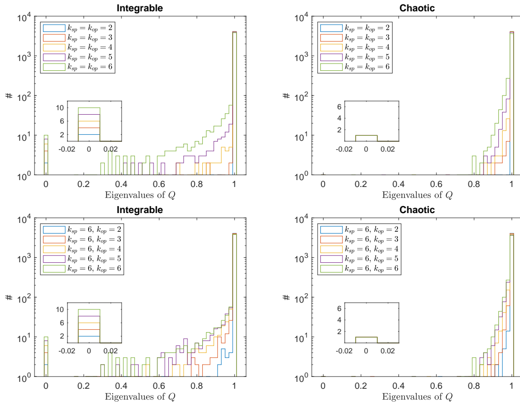
Figure 2: Histograms of the eigenvalues of the Q -matrix for Left column: an integrable Ising spin chain (57) with (h_x, h_z) = (-1.05, 0) and Right column: a chaotic Ising spin chain with (h_x, h_z) = (-1.05, 0.5) for varying locality thresholds as Top row: k_{sp} = k_{op} or Bottom row: only varying k_{op} while keeping k_{sp} = 6 fixed. The length of the chain is set to L = 12 . In the bottom left inset of each plot we zoom in on the size of the kernel of the Q -matrix. It can be seen that in the integrable case, the number of zero eigenvalues increases in steps of 2, in accordance with the form of the conserved charges (63)-(66).
