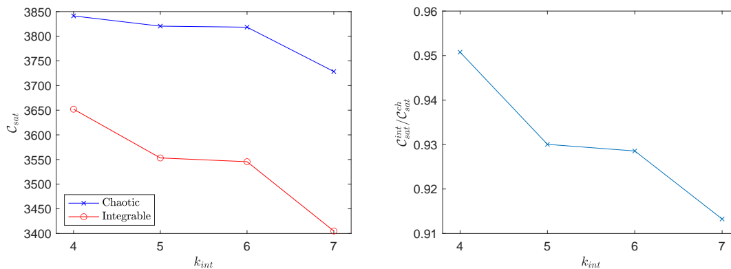
Figure 13: Left: Saturation values of the complexity bound as a function of k_{int} , with k_{sp} = k_{op} = \lceil k_{int}/2 \rceil , for the non-integrable (78) and integrable (82) spin 1 Hamiltonians. The length of the chain is set to L = 7 . Right: In order to highlight the complexity reduction of the integrable model, we display the ratio between the integrable and non-integrable curves on the left plot.
