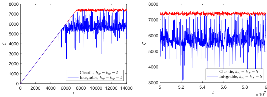
Figure 1: Left: The time evolution of the upper bound on Nielsen’s complexity for the Hamiltonian evolution of the transverse Ising model at (h_x, h_z) = (-1.05, 0) (blue) and the Ising model evaluated at a chaotic parameter point (h_x, h_z) = (-1.05, 0.5) (red). The length of the chain is L = 12 . To avoid using candidate minima that are evidently sub-optimal in estimating the complexity (26), at every time step we compare the output of the minimization procedure to the complexity associated to the early time solution k_n = 0 and the minimum of the two is chosen. Right: A zoom on the time window inside the plateau region used in the numerics.
