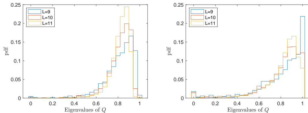
Figure 10: Histograms of the eigenvalues of the Q -matrix for Left: the chaotic Ising model (57) with (h_x, h_z) = (-1.05, 0.5) for L = 9, 10, 11 and fixed N_{loc}/D^2 = 0.15 . For the purpose of comparing the concentration properties of the distribution at varying L , we normalize the distributions so that the area below all the staircase curves is unity. The peak of the distribution can be seen to be close to 0.85, as expected from (44). Right: The same histograms for the transverse Ising at (h_x, h_z) = (-1.05, 0) , for comparison.
