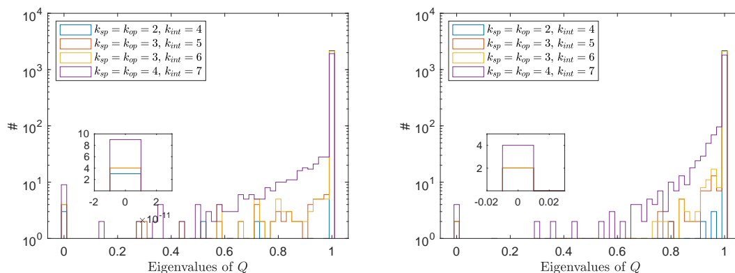
Figure 12: Histograms of the eigenvalues of the Q -matrix for Left : the integrable spin 1 XXX model (82) and Right : the non-integrable spin 1 XXX model (78) at L = 7 .
