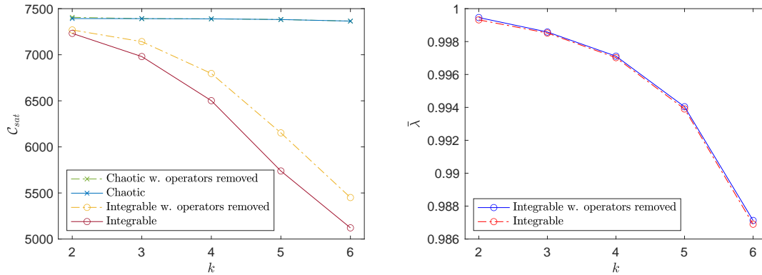
Figure 8: Left: Saturation values of the complexity bound as a function of k for a set of local generators \mathcal{T}_1 , with and without the operators (73). This is displayed for chaotic and integrable instances of the Ising model at L = 12 . Right: The mean of the Q -eigenvalue distributions shown in the left plot of Figure 7 and the upper left plot of Figure 2.
