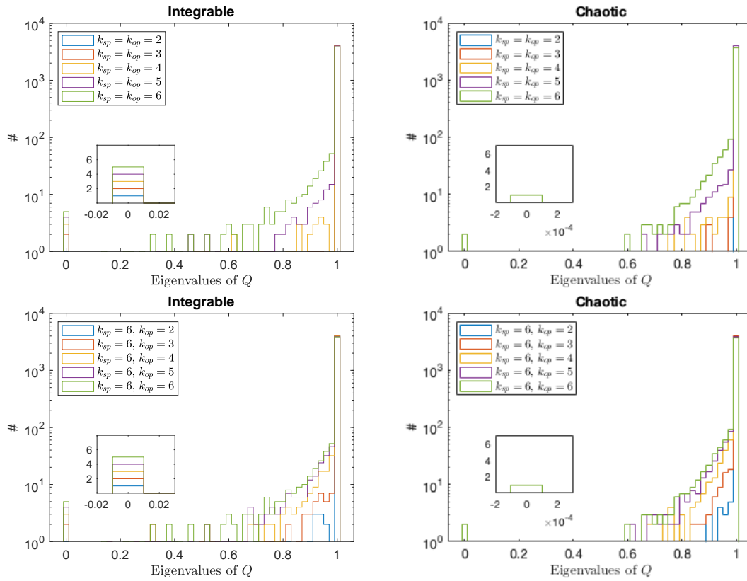
Figure 5: Histograms of the eigenvalues of the Q -matrix for the L = 12 Left column : integrable XYZ model (67) and for the Right column : chaotic XYZ model with magnetic field (72) (right) for varying locality thresholds as Top row : k_{sp} = k_{op} or Bottom row : only varying k_{op} while keeping k_{sp} = 6 fixed. For the coupling constants we used the numbers (J_x, J_y, J_z) = (-0.35, 0.5, -0.1) and on the right plot we chose h_z = 0.8 . In the bottom left corner of each plot we zoom in on the zero eigenvalues. The number of zero Q -eigenvalues in the integrable case increases in accordance with the form of the conserved charges.
