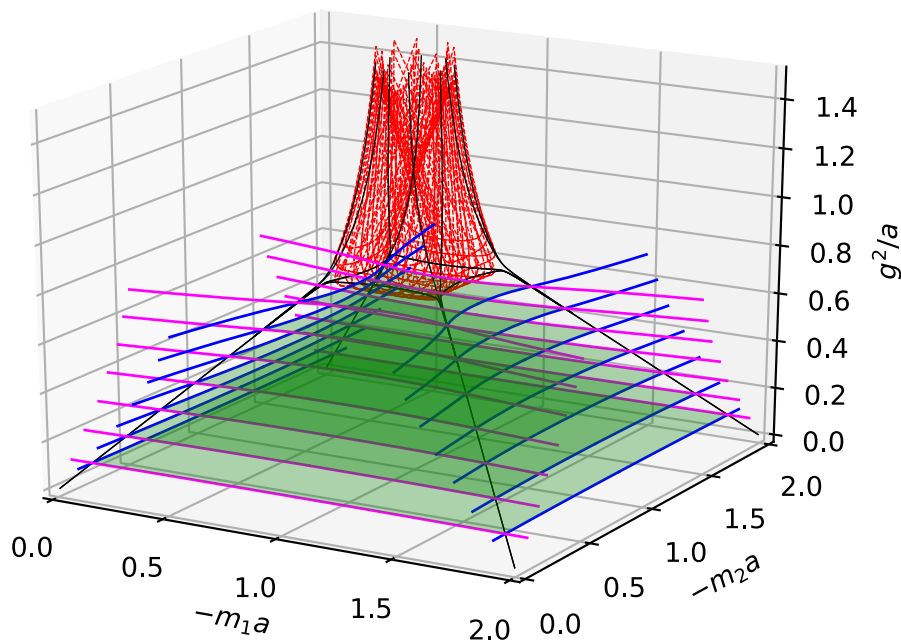
Figure 5: Interacting higher-order topological phase diagram I: We consider parameter space (m_1 a, m_2 a, g^2/a) , and represent the different phases in the twisted-Wilson lattice model with 4-Fermi interactions. The blue and magenta curves (74) delimit the inner green area (73) at fixed- g^2 slices that has a non-trivial many-body topological invariant e^{i\pi W_1(\Sigma)W_2(\Sigma)} = -1 for an odd number of fermion flavours. The red lines are obtained by solving the gap equations to localise the boundary of the parity-breaking \Pi condensate (71)-(72). The black lines demonstrate that this pseudo-scalar condensate actually grows from the four corners of the non-interacting HOTI phase at g^2 = 0 (see Fig. 4), forming the shape of an Eiffel tower that rests on the correlated HOTI. All numerical evaluations employed a spatial lattice with N_s = 32^2 sites.
