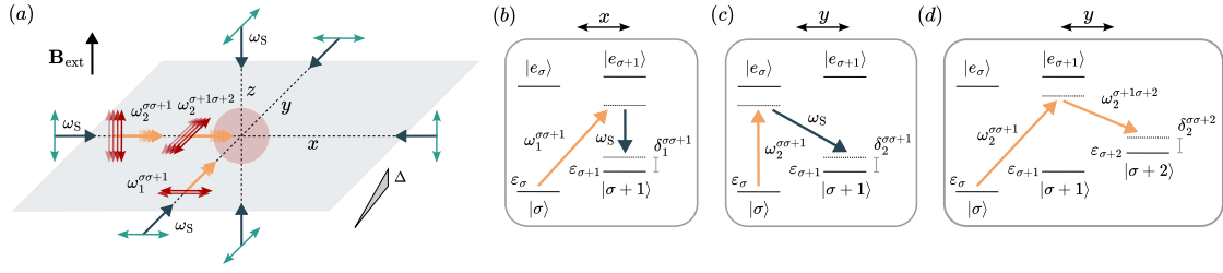
Figure 2: Raman optical lattice: (a) The atom cloud (light red sphere) is subjected to a 3D optical lattice, created using three pairs of counter-propagating laser beams (blue arrows) with mutually orthogonal polarizations (green arrows) and frequencies \omega_s . The atoms can be then confined into a 2D plane by increasing the potential depth in the z direction. Additionally, travelling Raman beams (orange arrows) with frequencies \omega_j^{\sigma\sigma'} and appropriate polarizations (red arrows) generate spin-changing processes, as discussed in the main text. Finally, a magnetic field \mathbf{B}_{\text{ext}} is applied in the z direction to split the hyperfine atomic energy levels, and a gradient obtained by lattice acceleration creates an energy difference \Delta between nearest-neighbour sites in the y direction. The panels (b), (c) and (d) depict the two-photon Raman transitions giving rise to spin-changing processes, where \varepsilon_\sigma is the electronic energy of |\sigma\rangle , and \delta_j^{\sigma\sigma'} the corresponding detunings.
