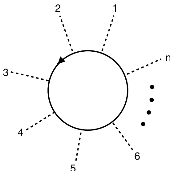
Figure 8: Large- N effective potential: Example of a Feynman diagram with n external zero-momentum auxiliary legs (dashed lines), and a single fermion loop (solid circle), yielding the main contribution to the effective potential V_{\text{eff}} in the large- N limit.
