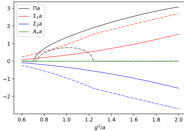
Figure 7: Competing condensation channels: Condensates as a function of g^2 for (m_1a, m_2a) = (-0.95, -1.05) (full lines) and (-0.85, -1.15) (dot-dashed lines). The opposite signs of \Sigma_1, \Sigma_2 mirror the signs of -1 - m_{1,2}a . Note that \mathbf{A} = \mathbf{0} throughout.
