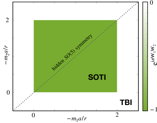
Figure 4: Non-interacting higher-order topological phase diagram: We represent the topological invariant in Eq. (45) as a function of the bare twisted masses m_1 and m_2 . In the green inner square m_j a \in (-2r, 0) , the topological invariant is non-trivial e^{i\pi W_1 W_2} = -1 , and the groundstate of the twisted-Wilson lattice model corresponds to a higher-order topological insulator (HOTI). The shaded line with m_1 = m_2 represents the regime where the model has a discrete SO(5) symmetry that protects the corner modes. The white region where m_j a \notin (-2r, 0) for one or both masses corresponds to a trivial band insulator (TBI) with trivial topological invariant e^{i\pi W_1 W_2} = +1 .
