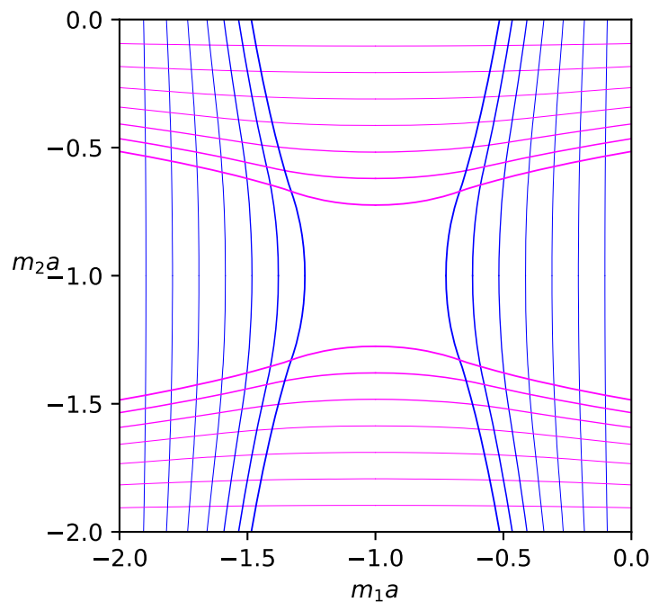
Figure 6: Interacting higher-order topological phase diagram II: Here the lines where the gap functions f_1 = 0 (blue) and f_2 = 0 (magenta) are plotted for increasing values of the coupling strength g^2/a \in \{0.1, 0.2, 0.3, 0.4, 0.5, 0.6, 0.7\} , which grow as one moves towards the center of the square. The HOTI phase is contained within a star-shaped region that is delimited by groups of four of these lines, corresponding to the same value of the coupling strength g^2/a .
