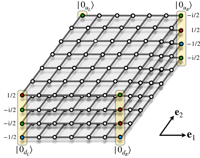
Figure 3: Anomalous corner states in the flat-band regime: For a finite multi-layer with parameters m_1 = m_2 = r/a and r = 1 , the Hamiltonian displays two-fold degenerate flat bands \epsilon_{q,\pm}(\mathbf{k}) = \pm 2t and four zero-energy modes (31) that are strictly localised to the corners of the lattice. The colouring of the sites at the corners corresponds to the complex phases of Eq. (31).
