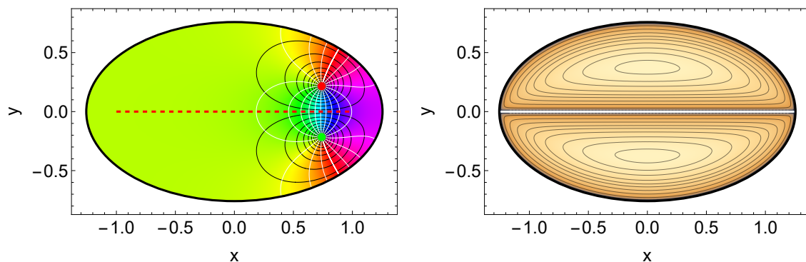
Figure 8: Left: streamlines (black lines) and phase (colour coding and white lines) associated with a symmetric vortex dipole inside the ellipse. This configuration consists of a positive vortex at position w_0 (red dot) and a negative one that is symmetric with respect to the focal line at position w_0^* (green dot). Right: constant-energy contours for the same symmetric vortex dipole. Colour coding is the same as in Fig. 5. The elliptical boundary has aspect ratio b/a = 0.6 .
