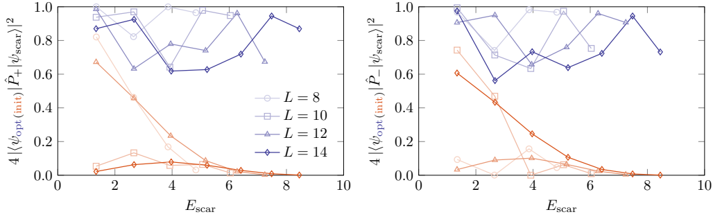
Figure 1: Blue lines (upper sets of curves) show the optimized overlaps 4|\langle \psi_{\text{opt}} | \hat{P}_{\pm} | \psi_{\text{scar}} \rangle|^2 (left panel) and 4|\langle \psi_{\text{opt}} | \hat{P}_{\pm} | \psi_{\text{scar}} \rangle|^2 (right panel) for several system sizes as a function of the energy of the quantum many-body scars. Red lines (lower sets of curves) show the overlap 4|\langle \psi_{\text{init}} | \hat{P}_{\pm} | \psi_{\text{scar}} \rangle|^2 (left panel) and 4|\langle \psi_{\text{init}} | \hat{P}_{\pm} | \psi_{\text{scar}} \rangle|^2 (right panel). The largest possible overlap with this normalization is unity.
