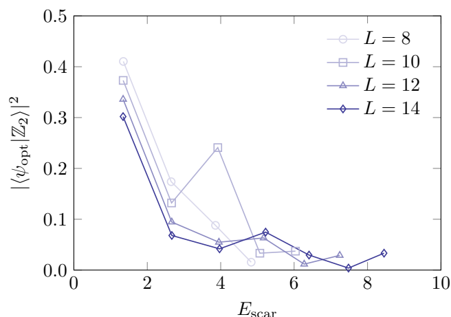
Figure 2: The overlap |\langle \psi_{\text{opt}} | \mathbb{Z}_2 \rangle|^2 as a function of the energy of the quantum many-body scars at several system sizes.
