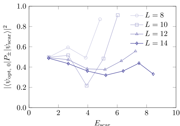
Figure 4: The optimized overlaps 4|\langle\psi_{\text{scar}}|\hat{P}_{\pm}|\psi_{\text{opt},0}\rangle|^2 for several system sizes as a function of the energy of the quantum many-body scars. The sign of the projector P_{\pm} is chosen such that it projects on to the parity sector containing the \mathbb{Z}_2 state. The largest possible overlap with this normalization is unity.
