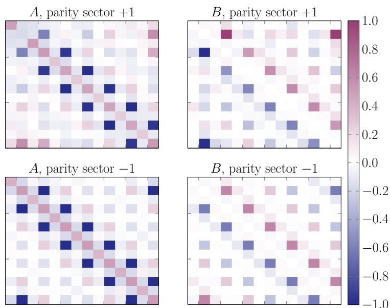
Figure 3: Color plots of the matrices A (left) and B (right) of the quadratic Hamiltonian (4), whose ground-state has the largest overlap with the scar with the second-highest energy for L = 14 . The top panels correspond to optimization with respect to \hat{P}_+|\psi_{\text{scar}}\rangle and the bottom panels with respect to \hat{P}_-|\psi_{\text{scar}}\rangle . The scale has been chosen such that the largest absolute value is unity.
