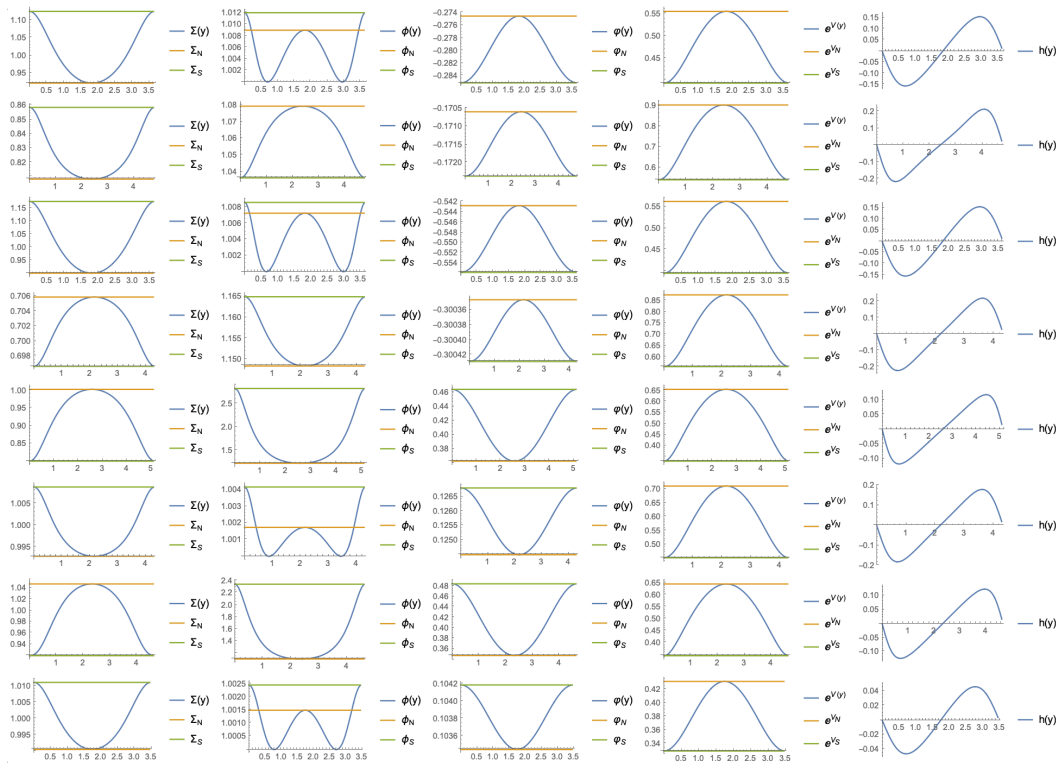
Figure 1: Numerical solutions for the scalar fields \Sigma(y) , \phi(y) , \varphi(y) and the scalar functions e^V(y) and h(y) interpolating between y = y_S = 0 and y = 2(y_N - y_S) . The values of n_S, n_N, p_F and \mathbf{z} are the ones fixed in (1). The values of the fields at y_S are the green lines and at y_N are the orange ones. From left to right, the plots follow the same order of table 1.
