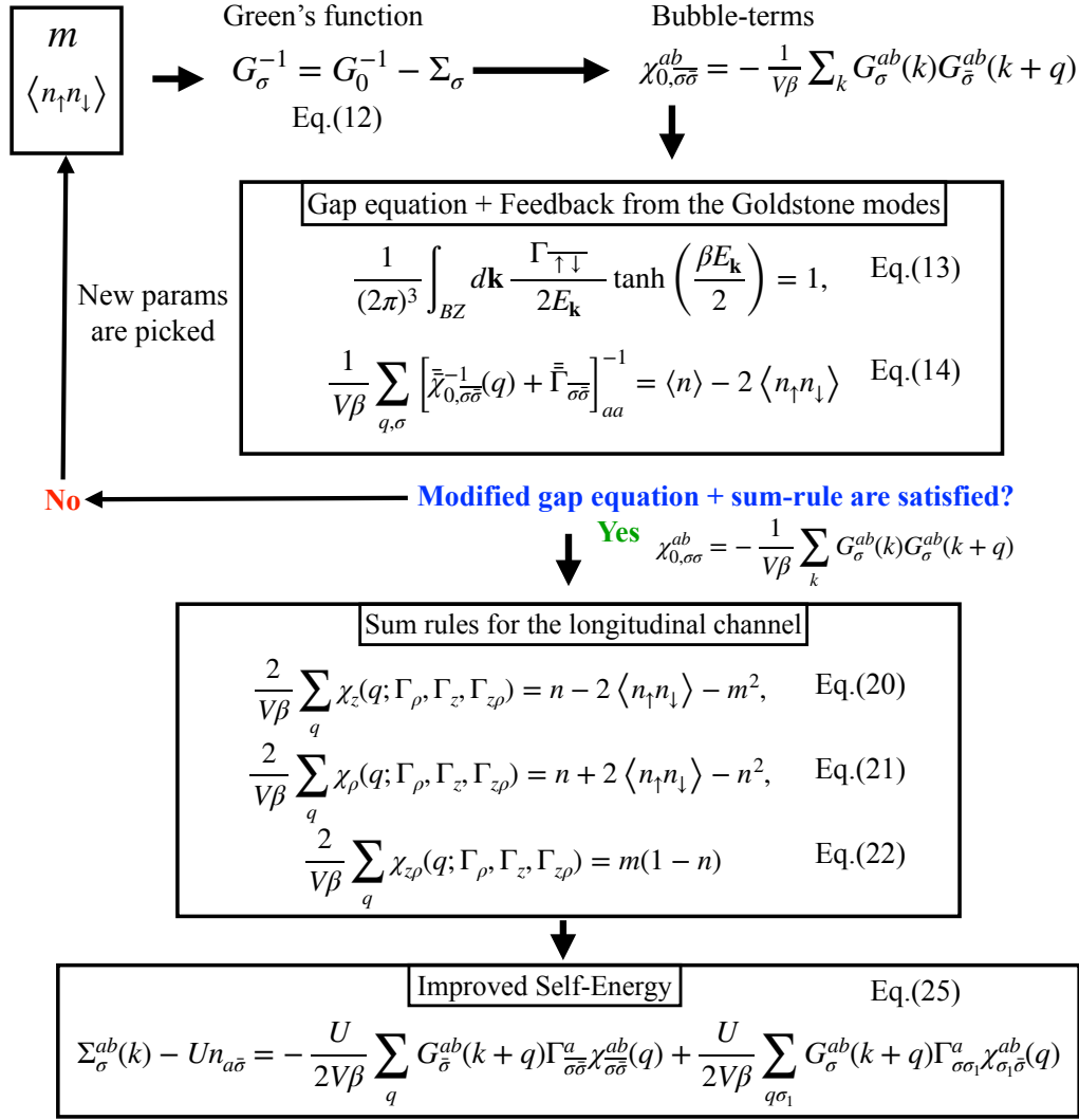
Figure 2: Work-flow of the Two-Particle Self-Consistent (TPSC) method for anti-ferromagnetic phases of the Hubbard model. The first box at the top shows how the staggered magnetisation m = n_{A\uparrow} - n_{A\downarrow} and double occupancies are obtained self-consistently by solving the gap equation [Eq. (13)] and the sum rule [Eq. (14)] for the spin-transverse channel, where Goldstone modes appear. An initial guess for m and \langle n_{\uparrow}n_{\downarrow} \rangle is used to calculate the Green's function and susceptibility. If Eqs. (13) and (14) are not satisfied, a minimisation routine adjusts the values. Once satisfied, the next step is to find the renormalised vertices in the spin-longitudinal channel by enforcing Eqs. (20), (21), and (22) shown in the middle box. With all renormalised interactions in the different channels, the improved electron self-energy can finally be computed using Eq. (25) displayed in the box at the bottom.
