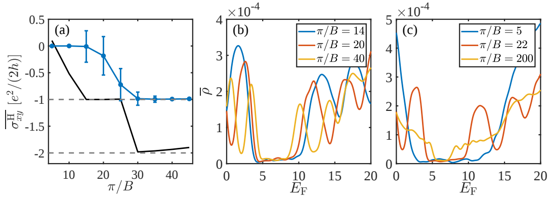
Figure 4: (a) Sample averaged Hall conductance \overline{\sigma_{xy}^H} with respect to the inverse of the magnetic field B at E_F = 12 for the regular lattice (black line) with L_x = 300, L_y = 20, L_z = 40 and amorphous lattices (blue line) with L_x = 200, L_y = 20, L_z = 40 . (b-c) Sample averaged DOS calculated under various magnitudes of the magnetic field.
