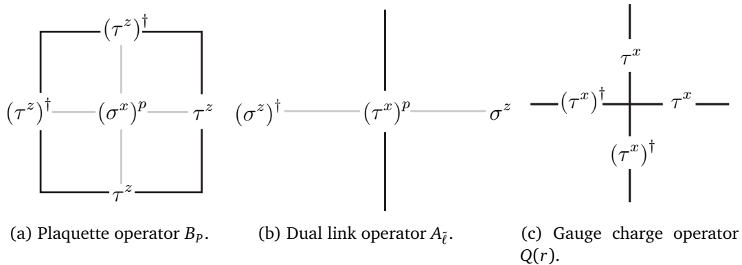
Figure 7: Depictions of (7a) the plaquette operator B_P , (7b) the dual link operator A_{\tilde{\ell}} , and (7c) the gauge charge operator Q(r) . The darker lines indicate links of the lattice while the lighter lines are links of the dual lattice.
