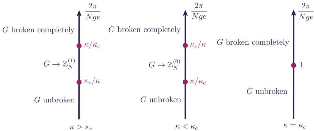
Figure 2: The phase diagram at \Theta = 0 for fixed \kappa = e/g as \text{Im}(\tau) = 2\pi/Nge is varied. In this limit, the lattice model reduces to a decoupled \mathbb{Z}_N clock model and \mathbb{Z}_N gauge theory. At large e and g , there is a trivial phase in which the clock model is disordered and the gauge theory is confining, fully preserving the global symmetry G = \mathbb{Z}_N^{(0)} \times \mathbb{Z}_N^{(1)} . At small e and g , the clock model orders, and the gauge theory is deconfined (and topologically ordered), breaking the full symmetry group G . Depending on the value of \kappa = e/g , there may be an intermediate phase in which either \mathbb{Z}_N^{(0)} or \mathbb{Z}_N^{(1)} is broken but not the other.
