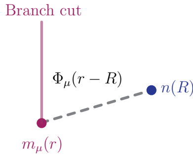
Figure 13: Statistical interaction in the Coulomb gas. The last term in the Coulomb gas action, Eq. (C.1), is a statistical interaction of spins and vortices. If m_\mu(r) is a straight line along the Euclidean time direction and n(R) is in the xy -plane, then \Phi_\mu(r - R) is the angle between the branch cut of m_\mu(r) and the shortest line from m_\mu(r) to n(R) .
