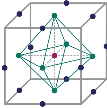
Figure 10: Depiction of the degrees of freedom in the lattice model, Eq. (162), on a single cube of the direct lattice. The \mathbb{Z}_N gauge field k_\mu(r) is defined on links \ell of the direct lattice, labeled by the blue points. The \mathbb{Z}_N spin variables k(R) are on sites R of the dual lattice, which are depicted by red points. The \mathbb{Z}_N axion \tilde{k}(\mathcal{R}) lives on the green points at the centers of plaquettes of the direct lattice. The green links connect nearest neighbors of sites \mathcal{R} where the \mathbb{Z}_N axion is defined.
