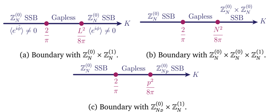
Figure 9: Examples of \mathbb{Z}_N^{(0)} \times \mathbb{Z}_N^{(1)} SPT boundary transitions captured by our gapless state, Eq. (130), as a function of the Luttinger parameter K if different global symmetries are preserved. In all cases, the gapless phase is Eq. (130), and the phase for K < 2/\pi has \mathbb{Z}_N^{(0)} symmetry breaking. If the only symmetry of the gapless theory preserved is the \mathbb{Z}_N^{(0)} \times \mathbb{Z}_N^{(1)} symmetry probed by the background fields, then for L = \gcd(N, p) \geq 4 , the gapless state is a critical point or line separating gapped phases of \mathbb{Z}_N^{(0)} symmetry breaking with different order parameters (9a). If we instead preserve the \mathbb{Z}_N^{(0)} \times \mathbb{Z}_N^{(0)} \times \mathbb{Z}_N^{(1)} subgroup (9b) or the \mathbb{Z}_{Np}^{(0)} \times \mathbb{Z}_N^{(1)} subgroup (9c) of the gapless phase, then we obtain \mathbb{Z}_N^{(0)} \times \mathbb{Z}_N^{(0)} or \mathbb{Z}_{Np}^{(0)} symmetry breaking phases respectively at large K .
