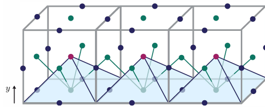
Figure 11: Depiction of the domain wall for the \mathbb{Z}_N axion. This domain wall is the non-invertible defect of Eq. (171). The vertical direction is the y -direction, and the plaquettes at the bottoms of the blue pyramids define the y = 0 plane. The y = 1/2 plane intersects the red points at the peaks of the pyramids. We have depicted three cubes, but of course, the domain wall extends infinitely in the imaginary time t and x directions. The domain wall lies on the blue triangles. The axion variables at the ends of the green links that intersect a blue triangle differ by a (\mathbb{Z}_N^{(0)})_{\text{axion}} transformation.
