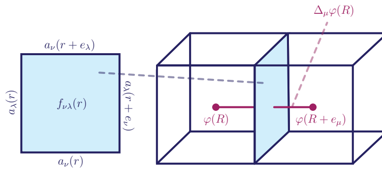
Figure 1: Depiction of the topological interaction on the lattice, Eq. (5). This (2+1)d analogue of the theta term represents an interaction of the field strengths, f_{\nu\lambda} , which are on plaquettes of the direct lattice, and spin phase variations, \Delta_\mu \varphi , which live on links of the dual lattice.
