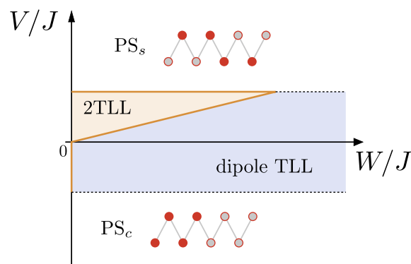
Figure 3: Simplified sketch of the phase diagram as obtained from the weak-coupling theory. Near the origin we find the 2TLL and dipole TLL phases. For large V these give room to phase separation \text{PS}_c and \text{PS}_s .
