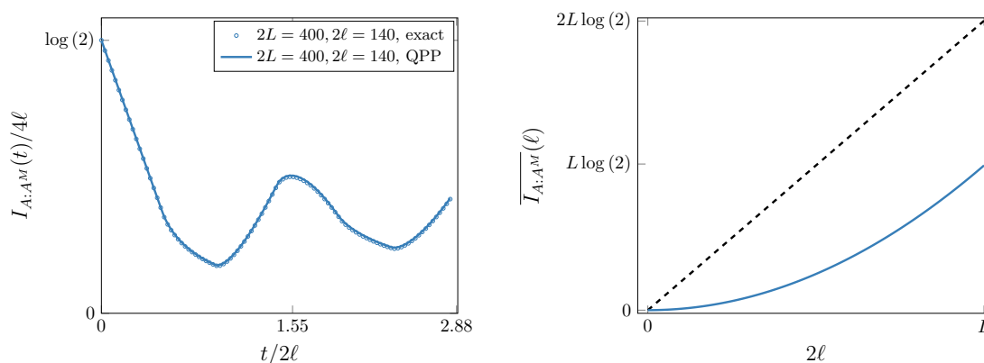
Figure 8: Left: I_{A:A^M}(t) , for total system size 2L = 400 and subsystem size 2\ell = 140 , with the symbols being the exact numerical result and the blue curve using the quasi-particle picture. Right: The time averaged mutual information \overline{I_{A:A^M}}(\ell) as a function of \ell \leq L/2 (solid blue). For comparison, we also plot the initial value I_{A:A^M}(0) (dashed black).
