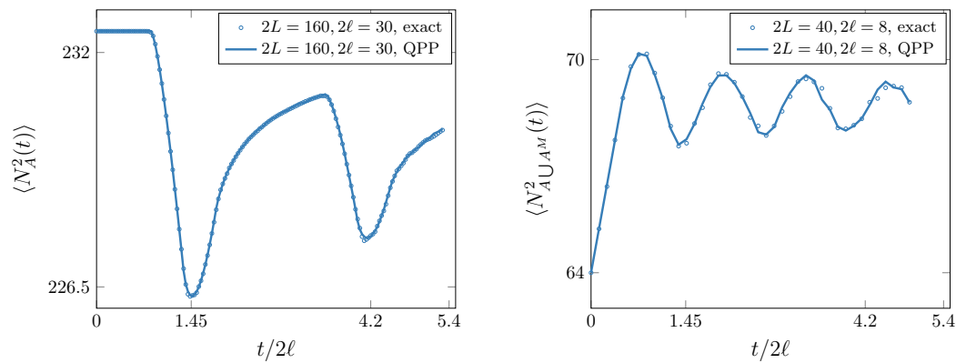
Figure 5: Left: \langle N_A^2(t) \rangle = \ell^2 + \sigma_A^2(t) for total system size 2L = 160 and subsystem size 2\ell = 30 , with the symbols being the exact calculation and the blue curve using the quasiparticle picture obtained from (68). Right: \langle N_{A \cup A^M}^2(t) \rangle , for total system size 2L = 40 and subsystem size 2\ell = 8 . The blue curve is given by (71) and the symbols are the exact numerical result.
