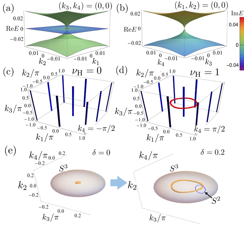
Figure 4: (a) and (b): Energy eigenvalues of Hamiltonian in Eq. (13) for m_0 = 3 and \delta = 0 . The real (imaginary) part is represented as height (color). In panel (b), complex conjugates of the upper and lower bands are omitted. (c) [(d)]: Lines in the momentum space (k_1, k_2, k_3) for m_0 = 3 , \delta = 0 and k_4 = -\pi/2 [ k_4 = \pi/2 ], where red and blue lines denote the momenta satisfying \mathbf{R} \propto (0, 0, 1)^T and \mathbf{R} \propto (0, 0, -1)^T , respectively. The linking of these lines determines the value of the Hopf invariant \nu_H . (e): Momenta satisfying \mathbf{R}(\mathbf{k}) = \mathbf{0} for k_1 = 0 and \delta = 0 resp. \delta = 0.2 (orange manifolds). As \delta is introduced, the symmetry-protected HEP4 inflates into a loop. The gray oval and the blue loop illustrate the S^3 resp. S^2 , both extending in the fourth dimension k_1 (not shown), on which one computes the Hopf invariant \nu_H resp. the resultant winding number W_2 (see Appendix A.2) [88].
