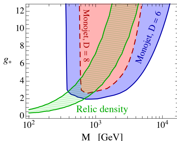
Figure 2: Same as in Fig. 1, but for fermionic Dirac DM. The region shaded in green corresponds to the observed relic abundance (fermionic DM comes with uncertainty about the chiral structure of the D = 6 effective operator considered [8], reflected by the width of the band, contrary to the single line of the scalar case).
