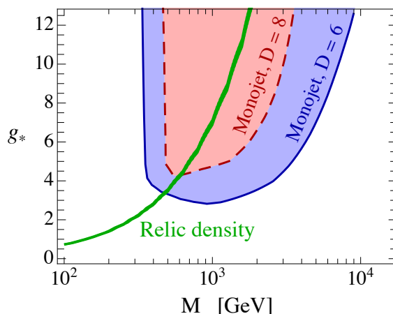
Figure 1: Constraints on scalar DM with m_{\text{DM}} = 5 GeV. Blue region: excluded by consistent LHC constraints on D=6 operator c_{\psi}^V in Eq. (4) (e.g. pseudo-NGB DM from a non-abelian SSB pattern), and comparison with the parameters where the RD is correctly reproduced with the same D=6 operator (solid green). Red region: LHC constraints on D=8 , C_{\psi}^T in Eq. (5) (e.g. one scalar DM from an abelian SSB).
