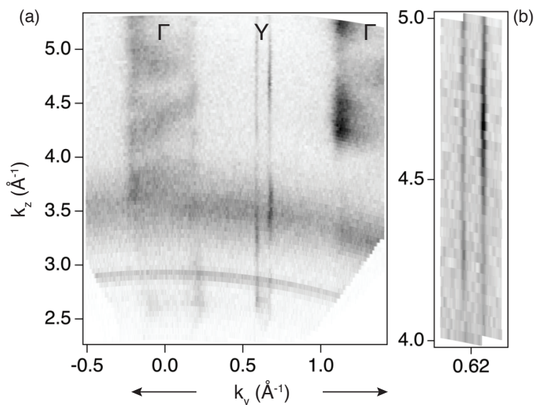
Figure 3: k_z -dependence of the electronic states. (a) k_z vs k_y intensity map for E=E_F for a \Gamma – Y cut, obtained from photon energy dependent ARPES experiments ( h\nu=20 - 120 eV). (b) Zoom-in on the Y state over a k_z region covering almost four Brillouin zones along k_z . It is clear that k_F for the Y -state shows little or no dependence on k_z , implying the quasi-2D nature of these states.
