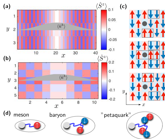
Figure 6: Precursors of stripe formation. We consider a single hole moving on the central chain of an n -leg ladder, described by the mixD t-J model with with open boundary conditions. We performed DMRG simulations for (a) an n = 3 -leg system with L_x = 40 sites in x -direction and (b) n = 5 and L_x = 10 . The hole density \langle \hat{n}_j^h \rangle forms a standing wave pattern with a pronounced maximum in the center of the middle chain (gray). The AFM order parameter \Omega_j = (-1)^{j_x + j_y} \langle \hat{S}_j^z \rangle changes sign in the center around j_x = L_x/2 . To understand this pattern from a parton perspective, one needs to consider multi-parton bound states. (c) In a three-leg ladder, the holon is bound to two spinons (domain walls) in the upper and lower chains. The possible spinon configurations (top and bottom) are coupled via a third state (center) with a spin-1 magnon excitation in the central chain. (d) The multi-parton state in the three-leg ladder is a generalization of a meson and can be understood as the analogue of a baryon. Similarly, the bound state in a five-leg ladder corresponds to a petaquark state.
