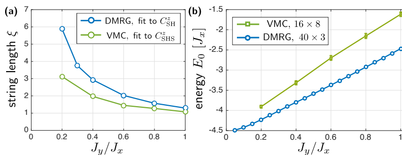
Figure 5: Dimensional crossover. We change from a 1D to a mixD situation by tuning J_y/J_x at t = 3J_x . (a) The string length \xi , extracted by fits of spin-hole correlators C_{SH}^z , sharply increases when J_y \rightarrow 0 . This indicates a deconfinement of the spinon-holon pair in this limit. (b) We compare the ground state energy E_0 of a single hole from DMRG in a 40 \times 3 system to the variational energy of the trial wavefunction in Eq. (4) in a 16 \times 8 system, evaluated at \mathbf{k}_{MP} = (\pi/2, \pi/2) , \Phi = 0.5\pi using VMC methods, see Methods for more details.
