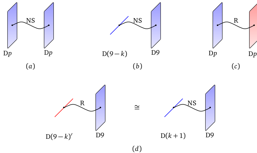
Figure 3: (a) A pair of Dp -branes with an NS sector string stretched between them; (b) an NS sector string stretched between a D(9 - k) - and D9 -brane; (c) an R sector string stretched between a Dp - and Dp' -brane; (d) an R sector string stretched between a D(9 - k)' - and D9 -brane, which can be thought of as an NS sector string stretched between a D(k + 1) - and D9 -brane, as far as the behavior of the fermion zero modes is concerned.
