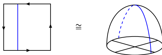
Figure 2: Projective plane with the single generator Z of its first homology class (in blue). To the right this is drawn as a sphere with a crosscap.
