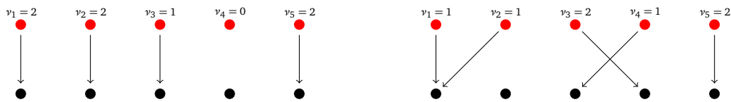
Figure 1: Sketch of two examples of a function f from p 's in red to q 's in black.
