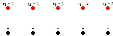
Figure 2: Sketch of configurations contributing to S_{0,0} .
