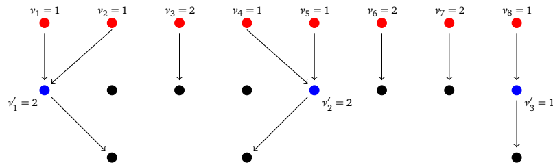
Figure 5: Sketch of the two functions f after one step of recursion. In red are indicated the p 's, in blue the q 's that play the role of the p 's after the first step of the recursion, that are those with index in I_1 or I_2 . The 'new' q 's on the last row are those with index in I_1 or I_0 .
