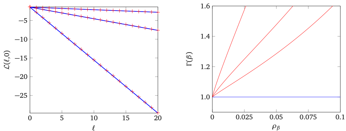
Figure 11: Left: \mathcal{L}(\ell, 0) for h = 0.5 and \beta = 2, 1, 0.25 (top to bottom). Numerical results for a L = 200 site open chain are shown as red crosses and equation (143) by a continuous blue line. Right: Numerically determined \Gamma(\beta) as a function of \rho_\beta for \ell = 30 and h = 3/4, 1/2, 1/4 from top to bottom; in blue is the expected value as \rho_\beta \rightarrow 0 .
