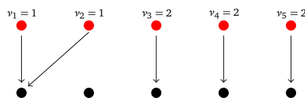
Figure 4: Sketch of configurations contributing to S_{0,2} .
