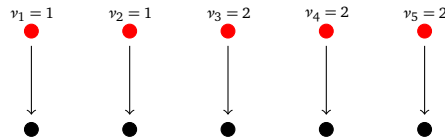
Figure 3: Sketch of configurations contributing to S_{2,0} .
