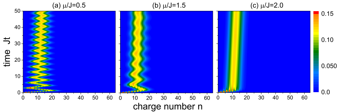
Figure 4: The dynamical evolution of the FCS P_n(t) of the charge number in half of the chain from an initial vacuum state. The parameters are: \Delta/J = 0.5, \gamma_-/J = 0.1, \gamma_+/J = 0.05 and N = 128 .
