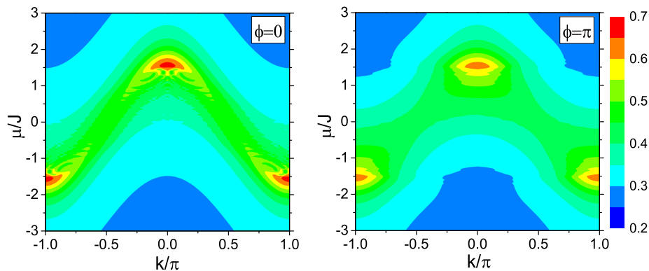
Figure 7: The k -distribution n(k) in the steady state with the statistical parameter \phi = 0 (left) and \phi = \pi (right). The other parameters \Delta, \gamma_{\pm} and N are the same as in Fig.1. The critical chemical potential is \mu_c/J = \pm 1.5 .
