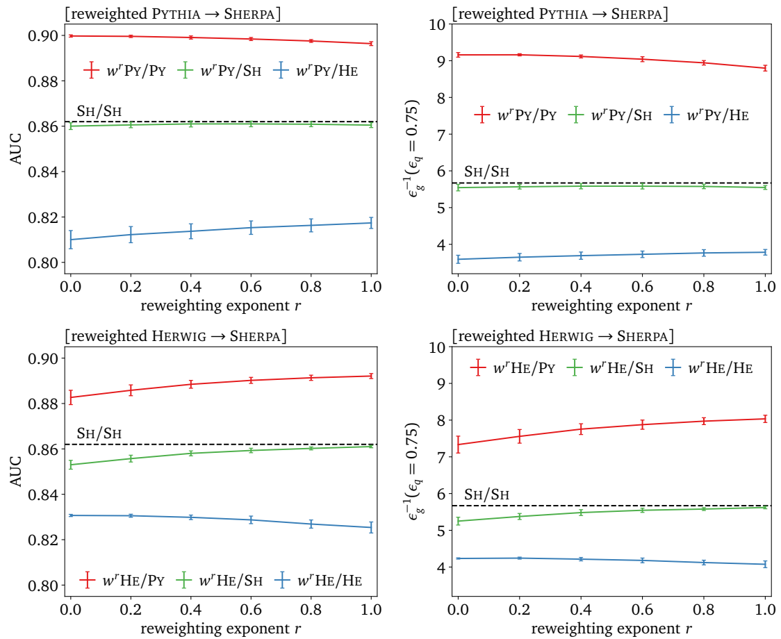
Figure 14: Performance of the interpolation between training and test data, using conditional reweighting PYTHIA → SHERPA ( upper ) and HERWIG → SHERPA ( lower ). The performance is benchmarked on pure HERWIG, PYTHIA, and SHERPA data. The error bars reflect six independent trainings.
