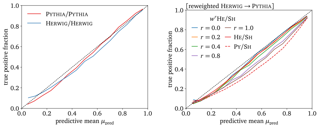
Figure 13: Left : calibration curves for consistent PYTHIA and HERWIG training and testing. Right : the same calibration curves using conditional HERWIG \rightarrow PYTHIA reweighting on the training data, tested on SHERPA. We also show the benchmark results from training on pure HERWIG and PYTHIA jets, corresponding to r \in \{0, 1\} .
