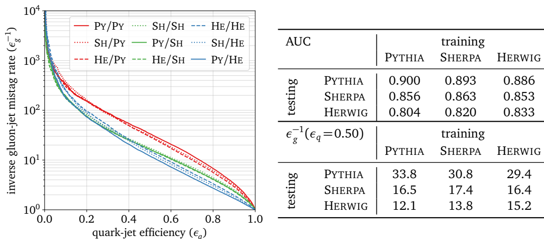
Figure 5: Left : ROC curves for training and testing on PYTHIA, SHERPA, and HERWIG in different combinations. Right : AUC and background-rejection performance of the BPN-Lite for quark-gluon tagging, trained and tested on the three different generators.
