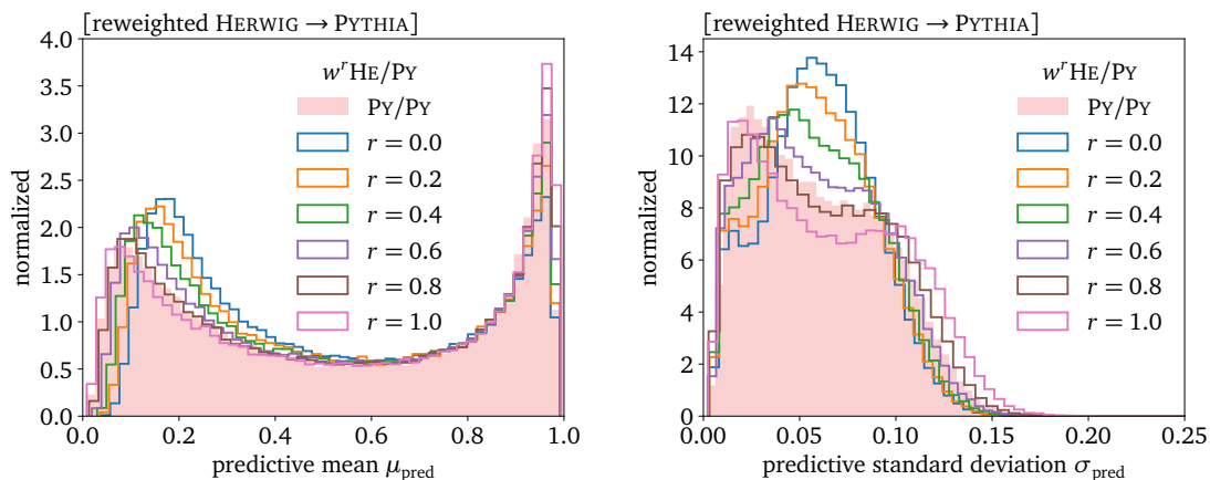
Figure 9: Bayesian ParticleNet-Lite, trained on reweighted HERWIG \rightarrow PYTHIA jets and tested on PYTHIA jets. The curves should be compared to those in Fig. 6.
