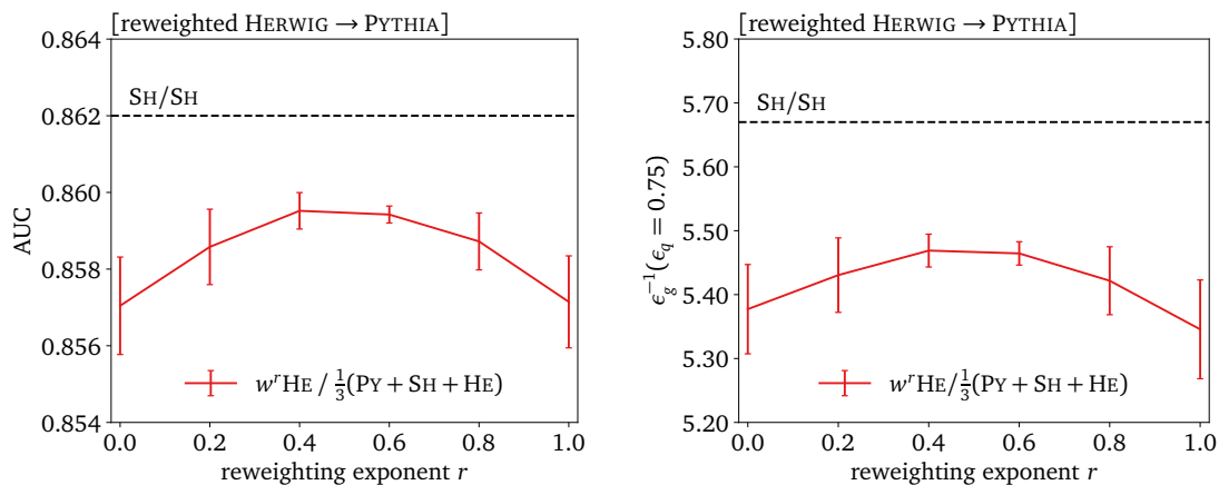
Figure 11: Performance of the interpolated training on HERWIG \rightarrow PYTHIA, using conditional reweighting. The performance is tested on equal parts of HERWIG, PYTHIA, and SHERPA jets. The error bars reflect six independent network trainings.
