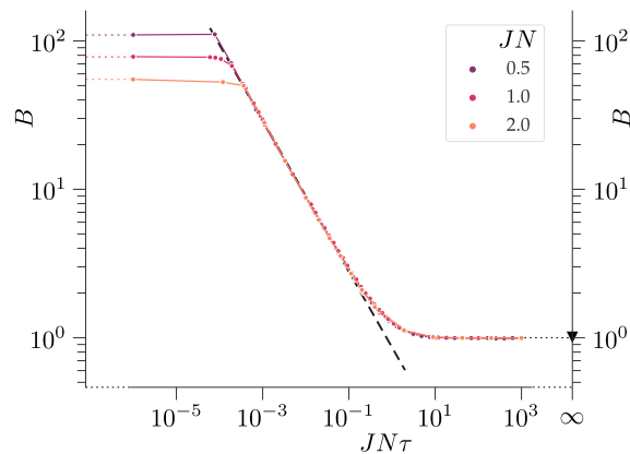
Figure 4: Parameter values yielding Born’s rule. The simulation is carried out for JN = 0.5 (dark), JN = 1 (middle), and JN = 2 (light). In each case, three regimes can be identified, corresponding to large, medium and small values of JN\tau . The dashed black line indicates a fit for the central regime, of the form B = \gamma/(JN\tau)^\alpha with \gamma \approx 0.92 and \alpha = 0.50 . The downward triangle on the right side indicates the exact result B = 1 for the limit JN\tau \rightarrow \infty , corresponding to constant noise or macroscopic measurement machines. The relation between JN\tau and B can be seen to become non-universal (dependent on JN ) for small values of JN\tau , where the approximation of a continuous noise process using finite step size breaks down. Each circular point along the curves represents the value of B giving Born’s rule as determined using a bisection method at fixed \theta_0 , and probabilities after averaging over 100000 evolutions using arc length steps of 0.05 for the noise.
