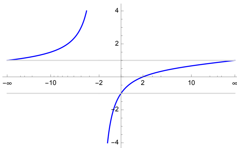
Figure 3: Plot of the \mu = 1 component of the SCT (29) with C^1 = -\frac{1}{2R} . We have set R = 1 for visualization purposes. The horizontal axis is the original Rindler coordinate X^1 , and the vertical axis is the transformed coordinate x^1 . Note that the entire right Rindler wedge, represented by the region X^1 > 0 , is mapped to the interval -R < x^1 < R (indicated by the gray horizontal lines), while the discontinuity at X^1 = -2R splits the left Rindler wedge over the complement.
