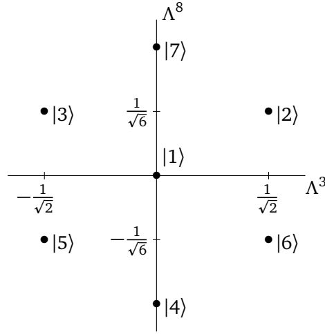
Figure 3: Weight diagram of the fundamental representation \mathbf{7} . The dots represent eigenstates |\sigma\rangle , \sigma = 1, \dots, 7 , of the two diagonal generators \Lambda^3 and \Lambda^8 , as fixed by the explicit matrix representation (A.2).
