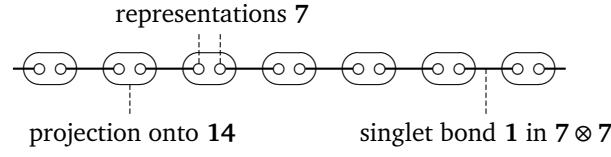
Figure 1: Graphical representation of the VBS state |\Psi_{\text{VBS}}\rangle . Each circle stands for a fundamental representation 7 , each line joining two circles for a singlet bond, i.e., the singlet 1 in the tensor product ( 1 ), and each oval for a lattice site on which we project onto the adjoint representation 14 .
