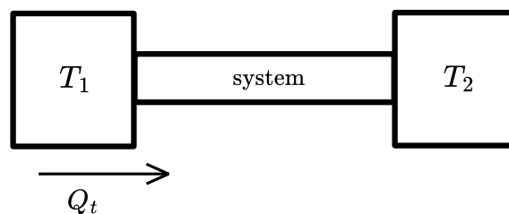
Figure 3: A system in contact with two heat baths. Q_t is the flux of particles from heat bath 1 to heat bath 2 during time t .
