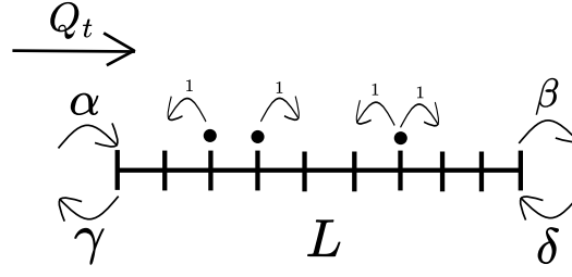
Figure 2: SSEP on L sites with open boundary conditions.
