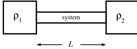
Figure 5: In diffusive systems, the transport coefficients \hat{\sigma} and \hat{D} decay like the inverse of the system size L .
