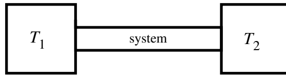
Figure 1: A system in contact with two heat baths at different temperatures.
