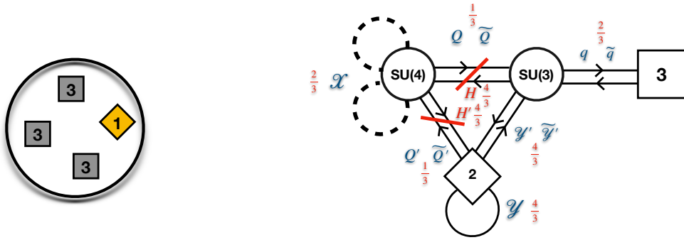
Figure 64: The theory corresponding to a sphere with three maximal punctures and one minimal puncture obtained by gluing to a T_3 the free trinion. On the right we have a non-conformal description of the theory using the Lagrangian of [82] for the T_3 . The fields H and H' are gauge singlets, and Y is adjoint of SU(2) . One maximal puncture SU(3) and the minimal puncture U(1) are manifest in the UV, while the remaining two maximal puncture SU(3) symmetries emerge in the IR enhancing an SU(2)^2 \times U(1)^2 symmetry of the Lagrangian. The U(1)_t symmetry is conjectured to emerge in the IR. One can further turn on marginal deformations consistent with the R-symmetry assignment in the Figure breaking completely all the global symmetry.
