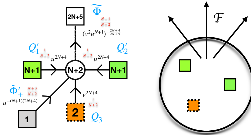
Figure 57: The three punctured sphere obtained by cutting the cycle of the one punctured torus. We have a baryonic superpotential \tilde{\Phi}'_+ \cdot (Q_1^{N+1} + Q_2^{N+1}) , which is irrelevant but the case of N = 1 . The trinion is associated to flux (-2, 0, \dots) which preserves U(1) \times SO(4N + 10) symmetry. The Figure is taken partially from [25].
