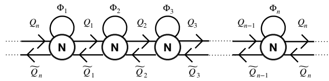
Figure 9: The necklace quiver of length n .
