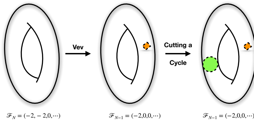
Figure 56: The sequence of operations: We start with a (D_{N+3}, D_{N+3}) torus with flux \mathcal{F}_N = (-2, -2, 0, \dots) preserving U(1) \times SO(4N + 8) \times SU(2) symmetry. We turn on then a vev to an operator which is charged under all three factors and breaks the symmetry to U(1)_{punct.} \times [U(1) \times SO(4N + 6)] and corresponds to the following flux of the IR theory, \mathcal{F}_{N-1} = (-2, 0, 0, \dots) . We obtain a torus with one puncture. The puncture parametrized by a combination of fugacities of the D_{2N+6} symmetry of the UV theory, U(1)_{punct.} , which are not parametrizing the D_{2N+4} symmetry of the IR 6d theory. Finally, we cut the torus along a cycle to obtain a sphere with two maximal and one minimal punctures with the flux equal to the one of the torus.
